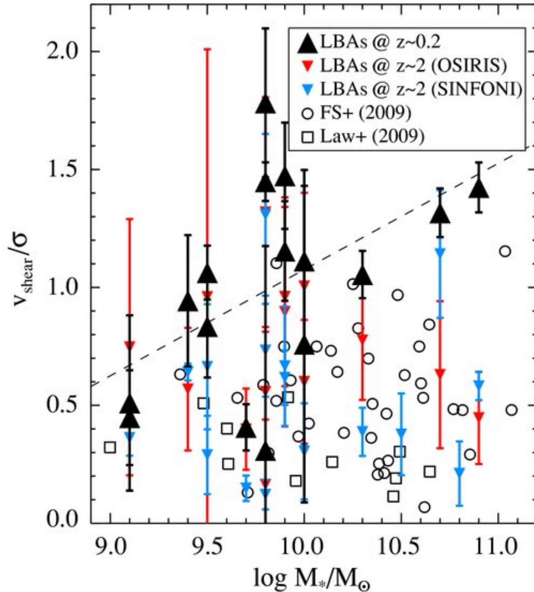
Figure 5. from The Kinematics of Ionized Gas in Lyman-break Analogs at z \sim 0.2 GONÇALVES ET AL. 2010 ApJ 724 1373 doi:10.1088/0004-637X/724/2/1373 https://dx.doi.org/10.1088/0004-637X/724/2/1373 © 2010. The American Astronomical Society. All rights reserved.
