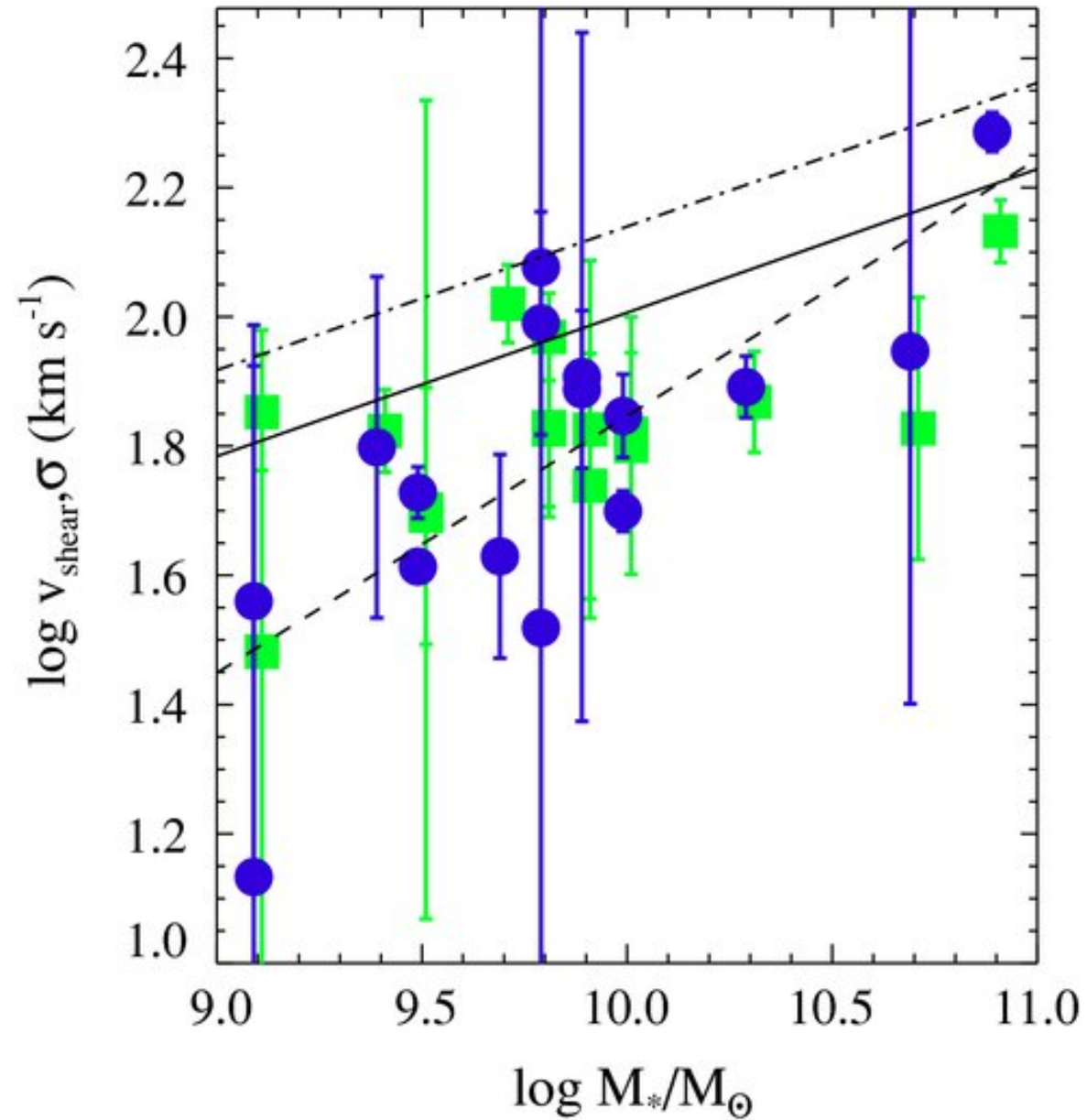
Figure 4. from The Kinematics of Ionized Gas in Lyman-break Analogs at z \sim 0.2 GONÇALVES ET AL. 2010 ApJ 724 1373 doi:10.1088/0004-637X/724/2/1373 https://dx.doi.org/10.1088/0004-637X/724/2/1373 © 2010. The American Astronomical Society. All rights reserved.
