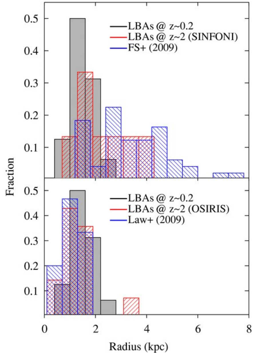
Figure 3. from The Kinematics of Ionized Gas in Lyman-break Analogs at z \sim 0.2 GONÇALVES ET AL. 2010 ApJ 724 1373 doi:10.1088/0004-637X/724/2/1373 https://dx.doi.org/10.1088/0004-637X/724/2/1373 © 2010. The American Astronomical Society. All rights reserved.
