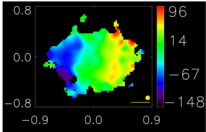
Figure 2. from The Kinematics of Ionized Gas in Lyman-break Analogs at z \sim 0.2 GONÇALVES ET AL. 2010 ApJ 724 1373 doi:10.1088/0004-637X/724/2/1373 https://dx.doi.org/10.1088/0004-637X/724/2/1373 © 2010. The American Astronomical Society. All rights reserved.
