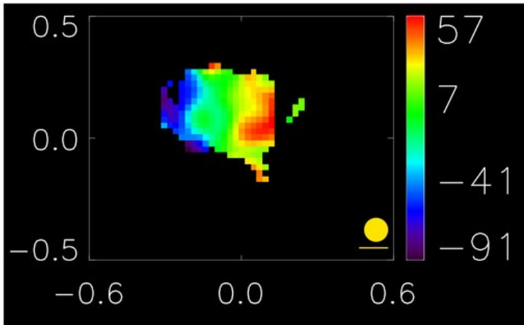
Figure 2. from The Kinematics of Ionized Gas in Lyman-break Analogs at z \sim 0.2 GONÇALVES ET AL. 2010 ApJ 724 1373 doi:10.1088/0004-637X/724/2/1373 https://dx.doi.org/10.1088/0004-637X/724/2/1373 © 2010. The American Astronomical Society. All rights reserved.
