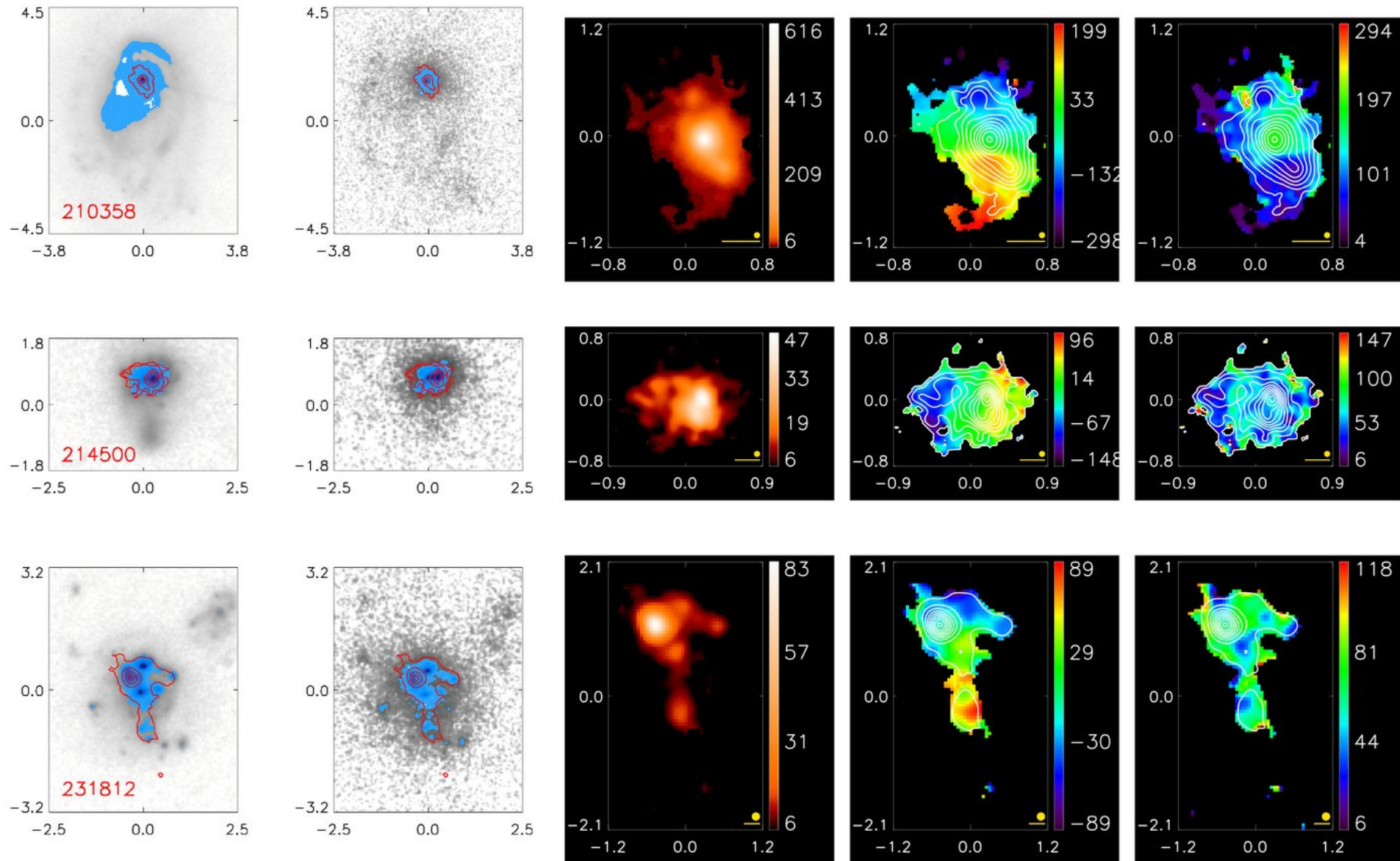
Figure 1. from The Kinematics of Ionized Gas in Lyman-break Analogs at z \sim 0.2 GONÇALVES ET AL. 2010 ApJ 724 1373 doi:10.1088/0004-637X/724/2/1373 https://dx.doi.org/10.1088/0004-637X/724/2/1373 © 2010. The American Astronomical Society. All rights reserved.
