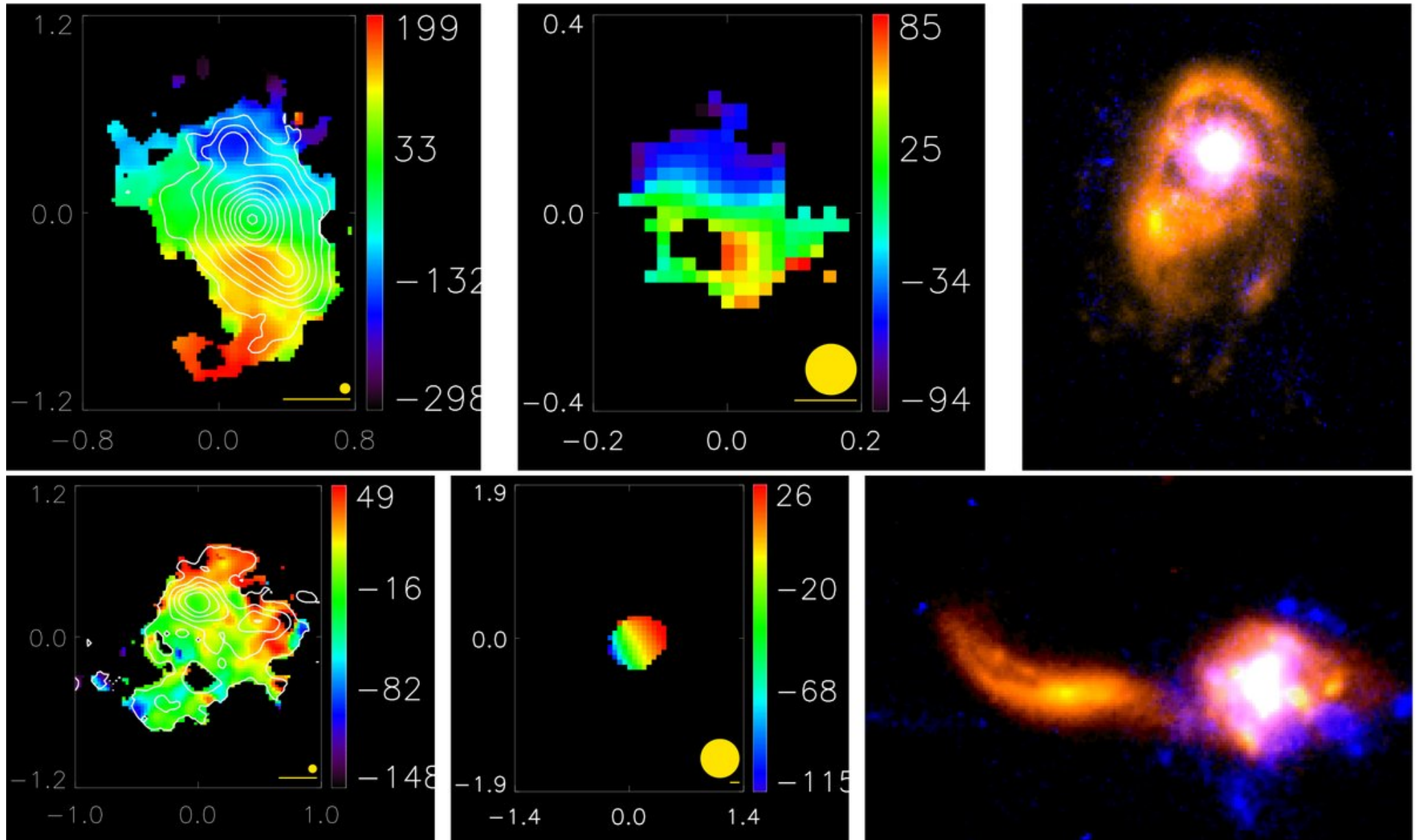
Figure 10. from The Kinematics of Ionized Gas in Lyman-break Analogs at z \sim 0.2 GONÇALVES ET AL. 2010 ApJ 724 1373 doi:10.1088/0004-637X/724/2/1373 https://dx.doi.org/10.1088/0004-637X/724/2/1373 © 2010. The American Astronomical Society. All rights reserved.
