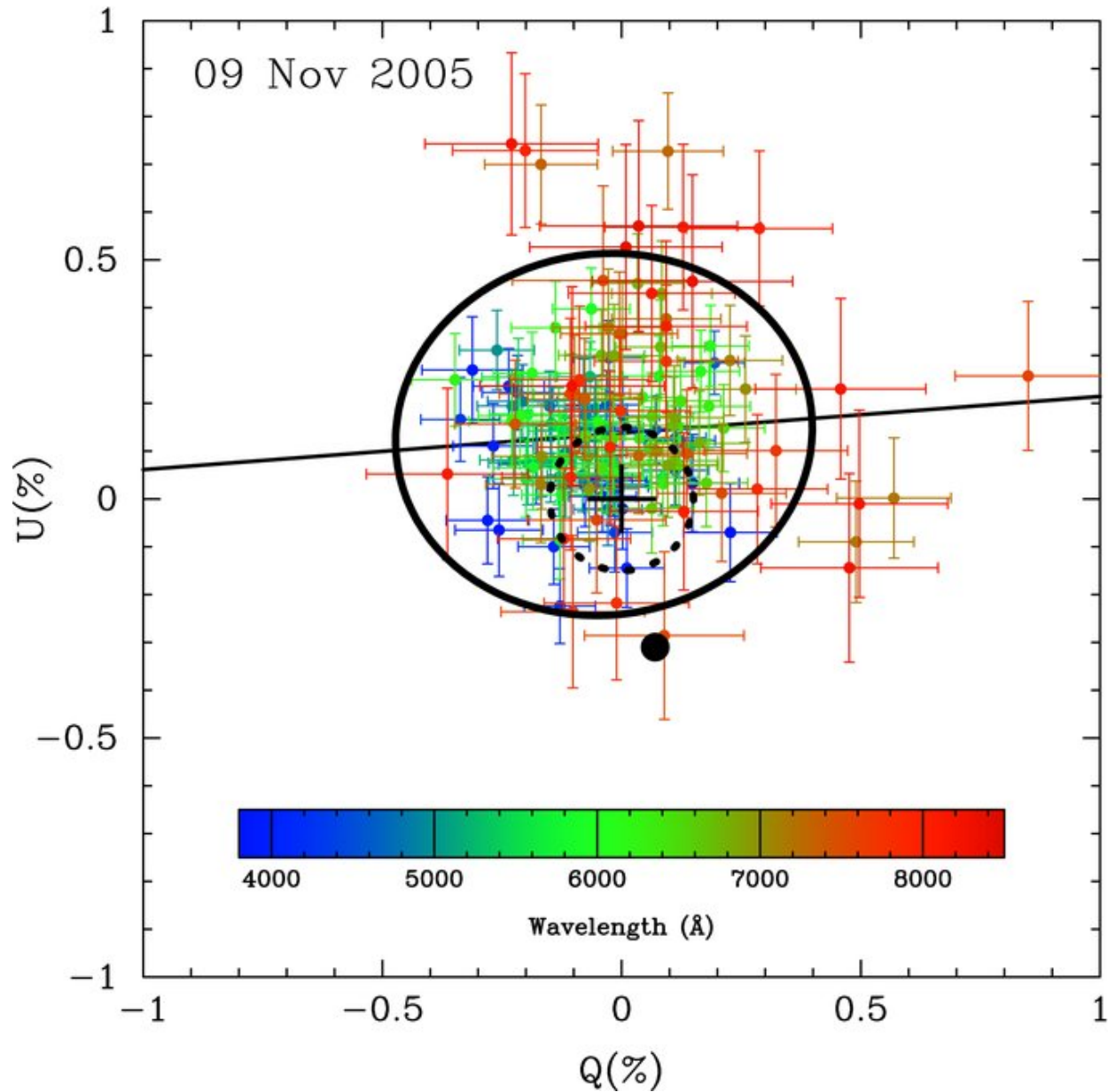
Figure 5. from A Spectropolarimetric View on the Nature of the Peculiar Type I SN 2005hk MAUND ET AL. 2010 ApJ 722 1162 doi:10.1088/0004-637X/722/2/1162 https://dx.doi.org/10.1088/0004-637X/722/2/1162 © 2010. The American Astronomical Society. All rights reserved.
