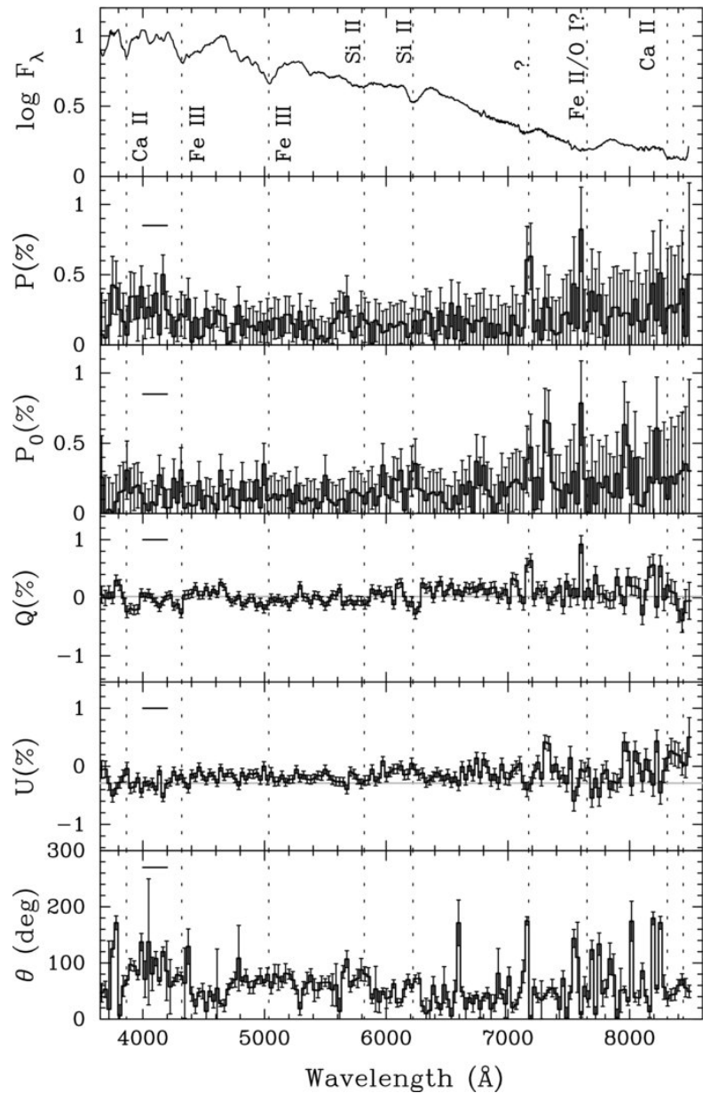
Figure 3. from A Spectropolarimetric View on the Nature of the Peculiar Type I SN 2005hk MAUND ET AL. 2010 ApJ 722 1162 doi:10.1088/0004-637X/722/2/1162 https://dx.doi.org/10.1088/0004-637X/722/2/1162 © 2010. The American Astronomical Society. All rights reserved.
