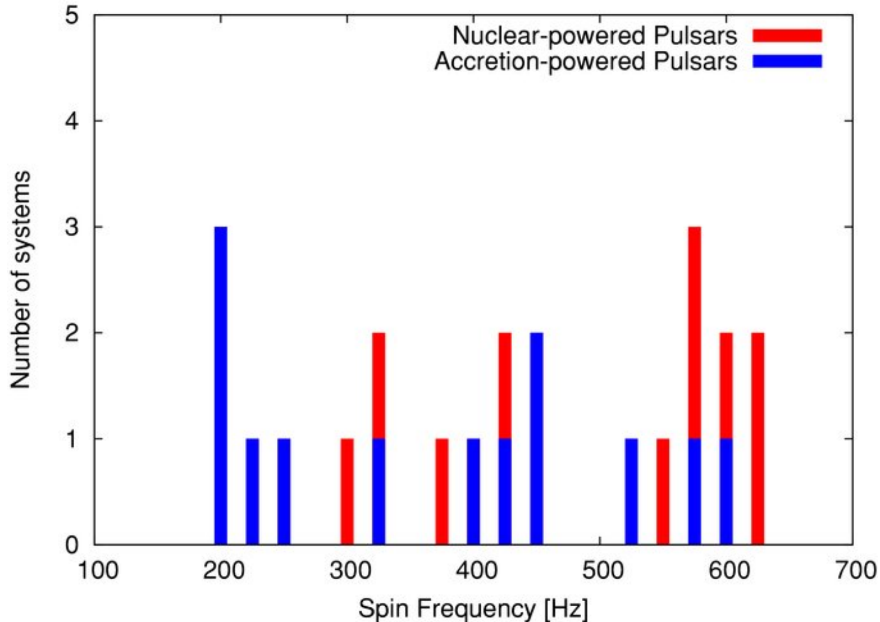
Figure 5. from The Accreting Millisecond X-ray Pulsar IGR J00291+5934: Evidence for a Long Timescale Spin Evolution PATRUNO 2010 ApJ 722 909 doi:10.1088/0004-637X/722/1/909 https://dx.doi.org/10.1088/0004-637X/722/1/909 © 2010. The American Astronomical Society. All rights reserved.
