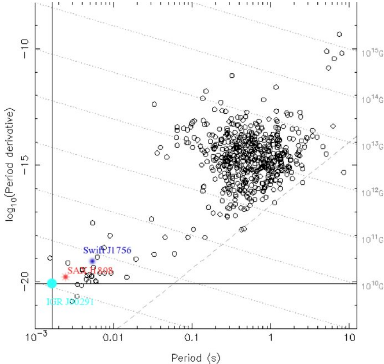
Figure 4. from The Accreting Millisecond X-ray Pulsar IGR J00291+5934: Evidence for a Long Timescale Spin Evolution PATRUNO 2010 ApJ 722 909 doi:10.1088/0004-637X/722/1/909 https://dx.doi.org/10.1088/0004-637X/722/1/909 © 2010. The American Astronomical Society. All rights reserved.
