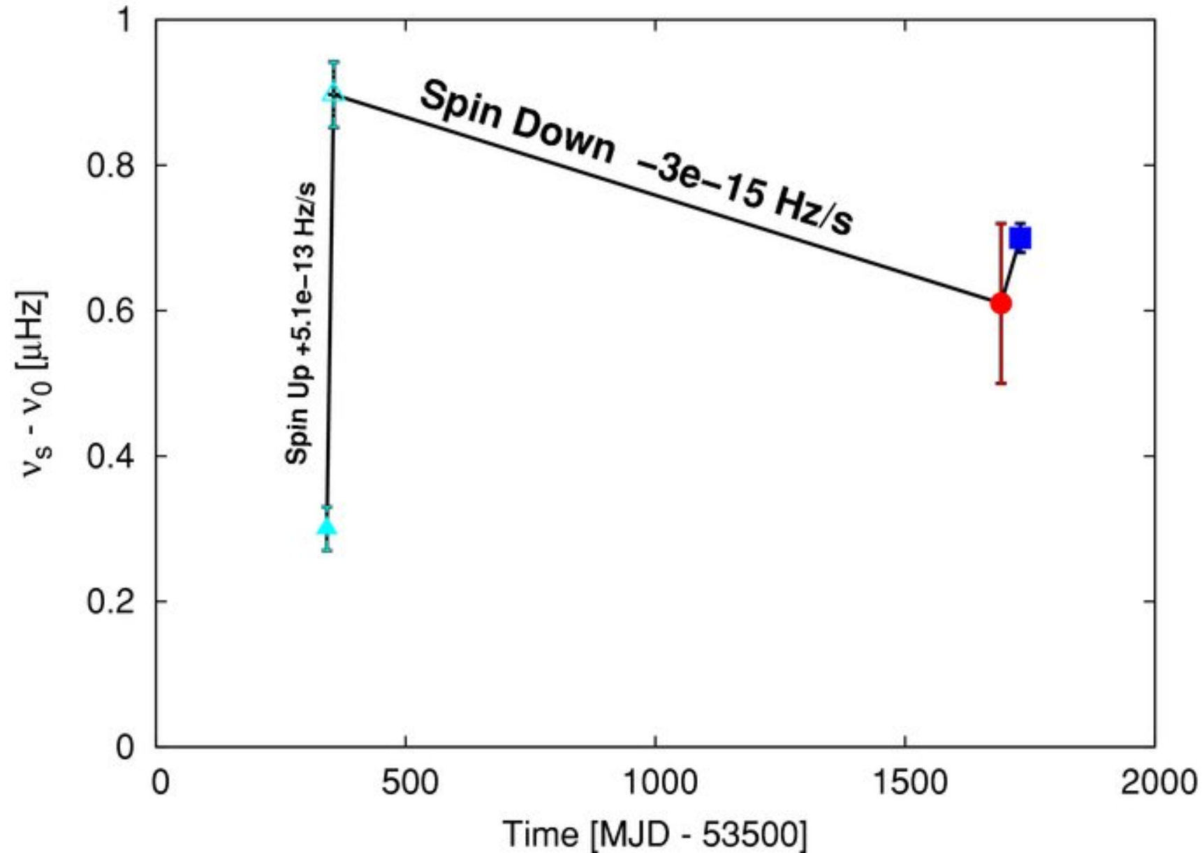
Figure 3. from The Accreting Millisecond X-ray Pulsar IGR J00291+5934: Evidence for a Long Timescale Spin Evolution PATRUNO 2010 ApJ 722 909 doi:10.1088/0004-637X/722/1/909 https://dx.doi.org/10.1088/0004-637X/722/1/909 © 2010. The American Astronomical Society. All rights reserved.
