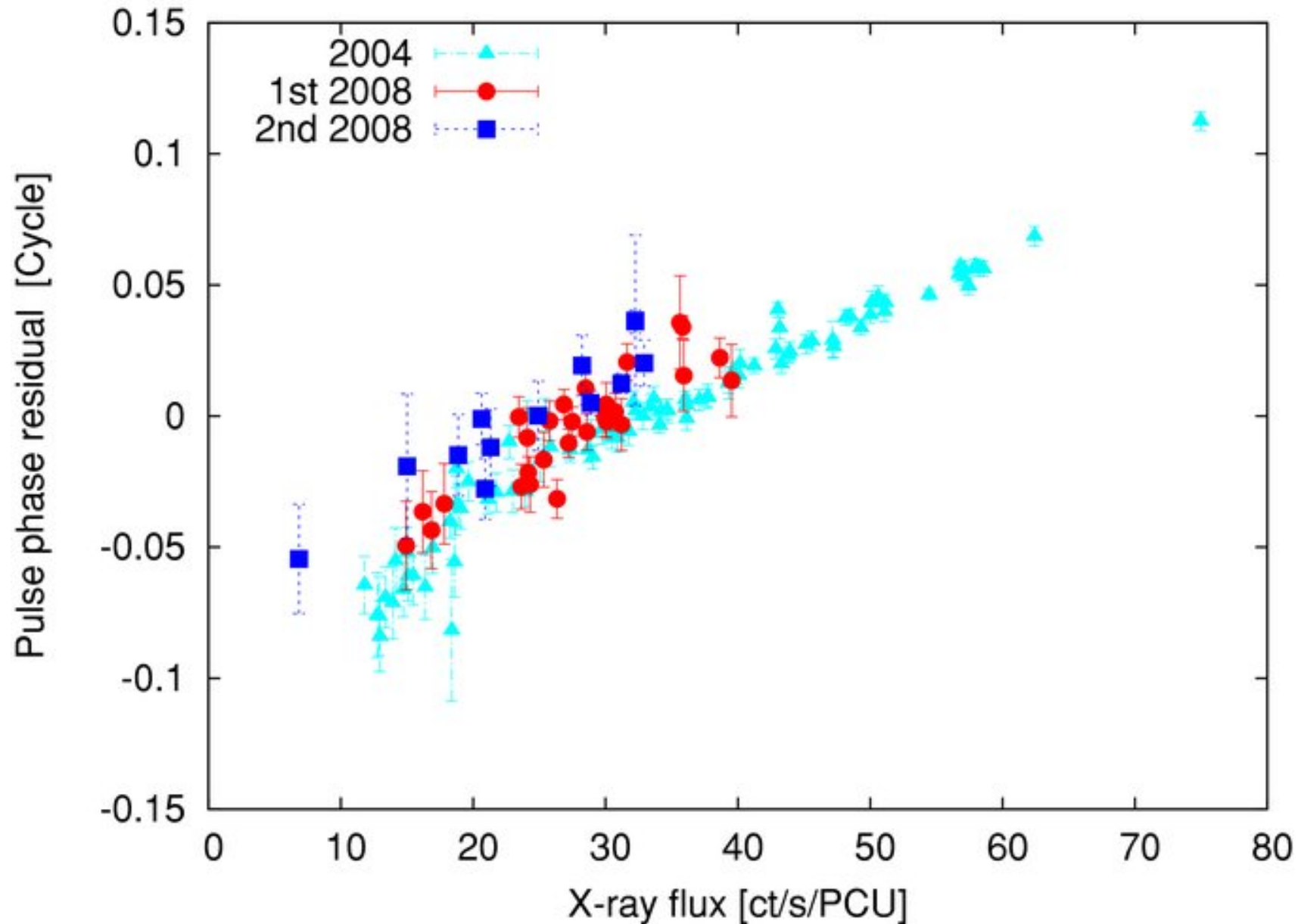
Figure 2. from The Accreting Millisecond X-ray Pulsar IGR J00291+5934: Evidence for a Long Timescale Spin Evolution PATRUNO 2010 ApJ 722 909 doi:10.1088/0004-637X/722/1/909 https://dx.doi.org/10.1088/0004-637X/722/1/909 © 2010. The American Astronomical Society. All rights reserved.
