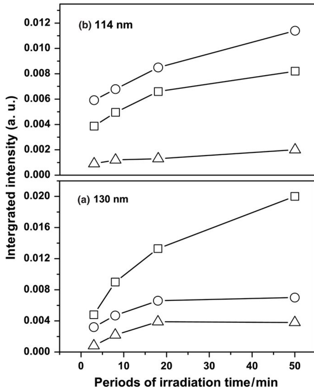
Figure 8. from Photolysis of Ethyne in Solid Neon and Synthesis of Long-chain Carbon Clusters with Vacuum-ultraviolet Light WU ET AL. 2010 ApJ 721 856 doi:10.1088/0004-637X/721/1/856 https://dx.doi.org/10.1088/0004-637X/721/1/856 © 2010. The American Astronomical Society. All rights reserved.
