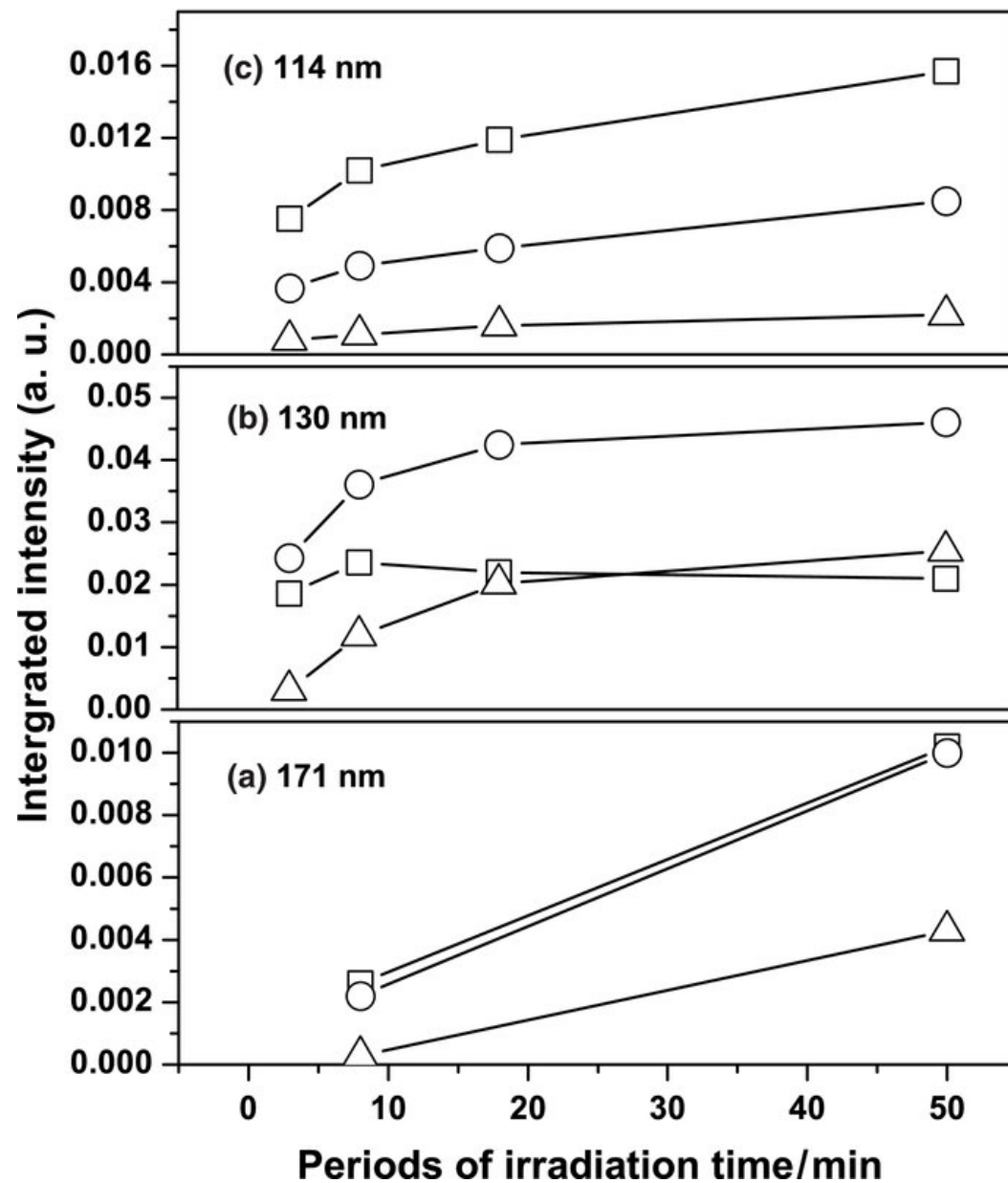
Figure 7. from Photolysis of Ethyne in Solid Neon and Synthesis of Long-chain Carbon Clusters with Vacuum-ultraviolet Light WU ET AL. 2010 ApJ 721 856 doi:10.1088/0004-637X/721/1/856 https://dx.doi.org/10.1088/0004-637X/721/1/856 © 2010. The American Astronomical Society. All rights reserved.
