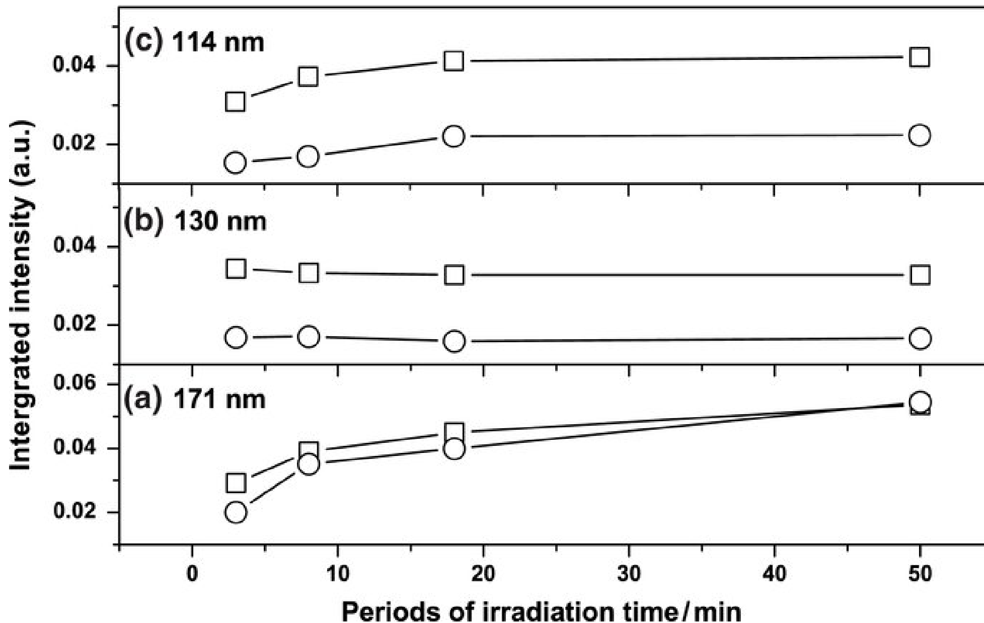
Figure 6. from Photolysis of Ethyne in Solid Neon and Synthesis of Long-chain Carbon Clusters with Vacuum-ultraviolet Light WU ET AL. 2010 ApJ 721 856 doi:10.1088/0004-637X/721/1/856 https://dx.doi.org/10.1088/0004-637X/721/1/856 © 2010. The American Astronomical Society. All rights reserved.
