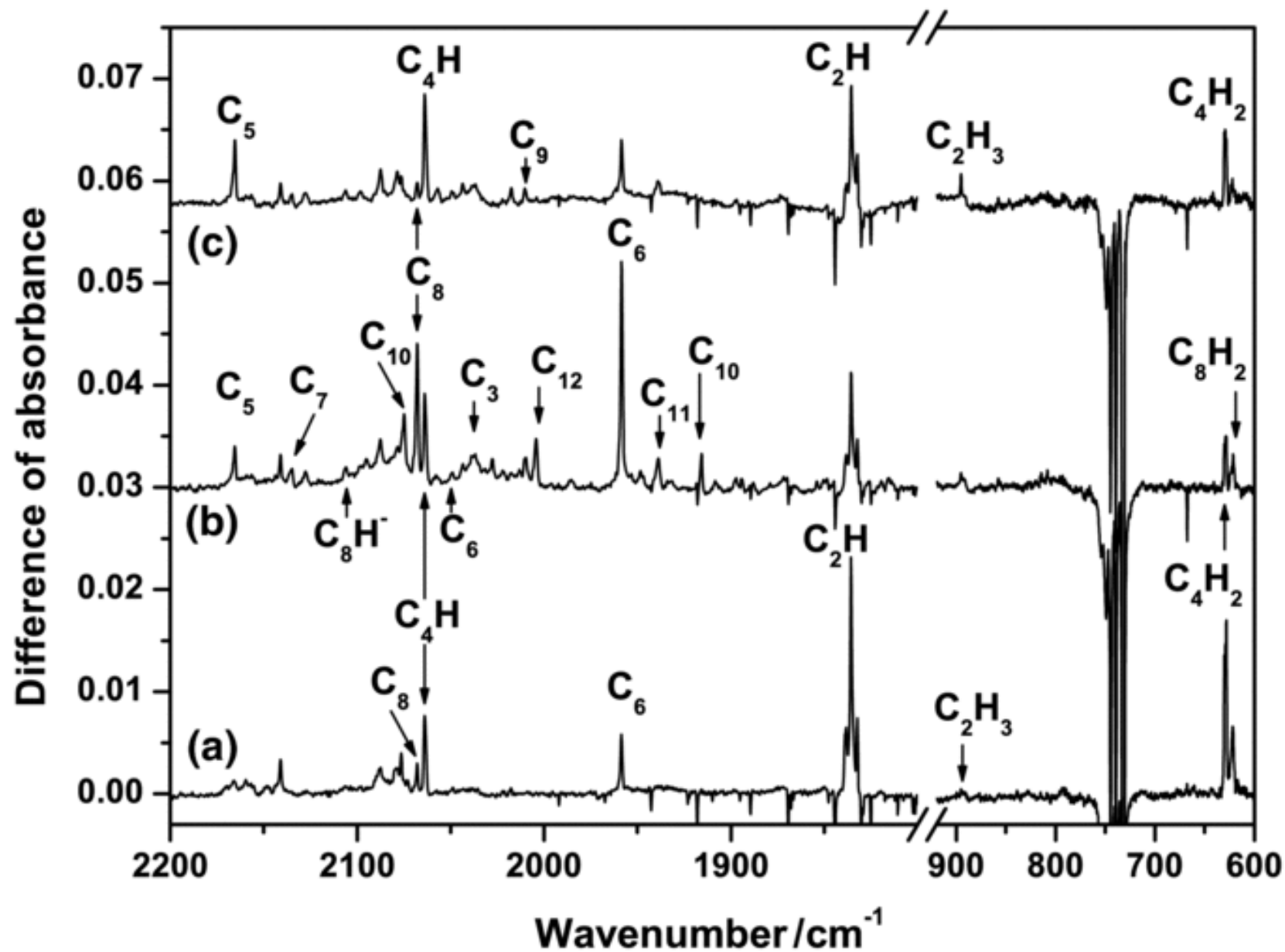
Figure 5. from Photolysis of Ethyne in Solid Neon and Synthesis of Long-chain Carbon Clusters with Vacuum-ultraviolet Light WU ET AL. 2010 ApJ 721 856 doi:10.1088/0004-637X/721/1/856 https://dx.doi.org/10.1088/0004-637X/721/1/856 © 2010. The American Astronomical Society. All rights reserved.
