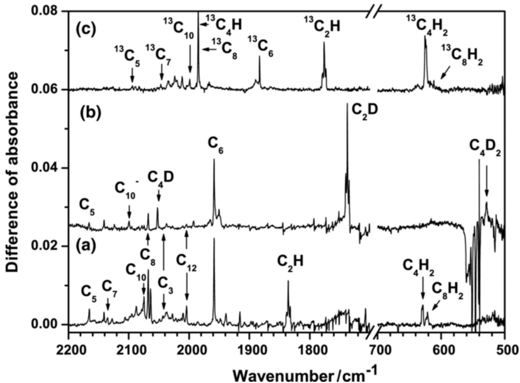
Figure 4. from Photolysis of Ethyne in Solid Neon and Synthesis of Long-chain Carbon Clusters with Vacuum-ultraviolet Light WU ET AL. 2010 ApJ 721 856 doi:10.1088/0004-637X/721/1/856 https://dx.doi.org/10.1088/0004-637X/721/1/856 © 2010. The American Astronomical Society. All rights reserved.
