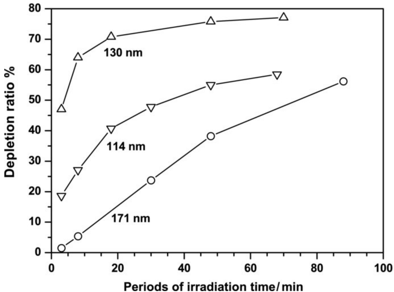
Figure 3. from Photolysis of Ethyne in Solid Neon and Synthesis of Long-chain Carbon Clusters with Vacuum-ultraviolet Light WU ET AL. 2010 ApJ 721 856 doi:10.1088/0004-637X/721/1/856 https://dx.doi.org/10.1088/0004-637X/721/1/856 © 2010. The American Astronomical Society. All rights reserved.
