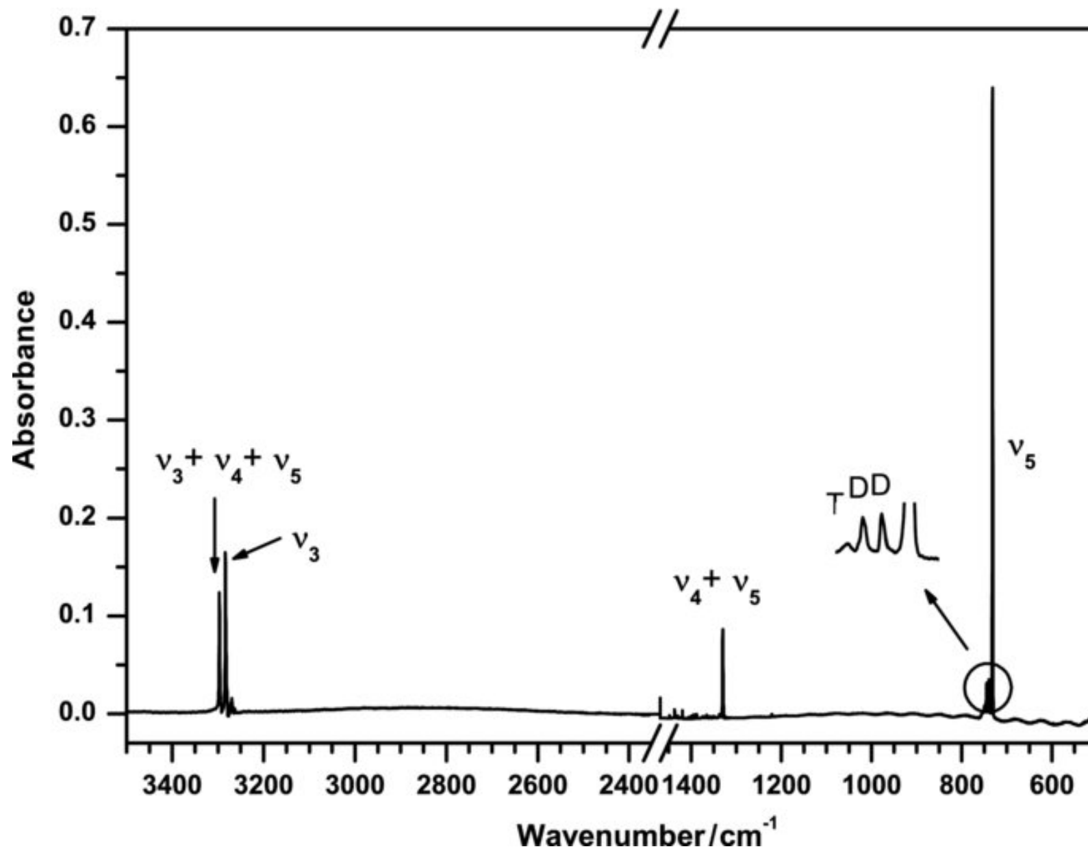
Figure 2. from Photolysis of Ethyne in Solid Neon and Synthesis of Long-chain Carbon Clusters with Vacuum-ultraviolet Light WU ET AL. 2010 ApJ 721 856 doi:10.1088/0004-637X/721/1/856 https://dx.doi.org/10.1088/0004-637X/721/1/856 © 2010. The American Astronomical Society. All rights reserved.
