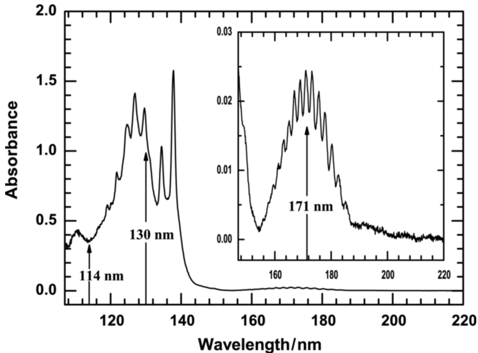
Figure 1. from Photolysis of Ethyne in Solid Neon and Synthesis of Long-chain Carbon Clusters with Vacuum-ultraviolet Light WU ET AL. 2010 ApJ 721 856 doi:10.1088/0004-637X/721/1/856 https://dx.doi.org/10.1088/0004-637X/721/1/856 © 2010. The American Astronomical Society. All rights reserved.
