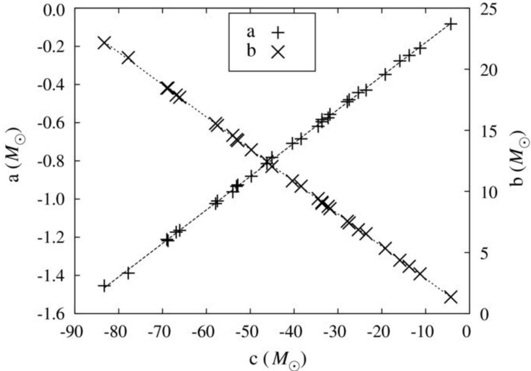
Figure 9. from Evaluating Systematic Dependencies of Type Ia Supernovae: The Influence of Deflagration to Detonation Density JACKSON ET AL. 2010 ApJ 720 99 doi:10.1088/0004-637X/720/1/99 https://dx.doi.org/10.1088/0004-637X/720/1/99 © 2010. The American Astronomical Society. All rights reserved.
