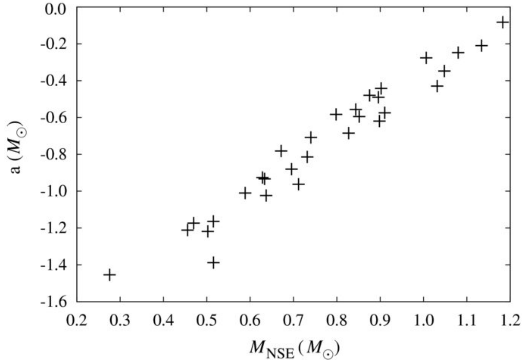
Figure 8. from Evaluating Systematic Dependencies of Type Ia Supernovae: The Influence of Deflagration to Detonation Density JACKSON ET AL. 2010 ApJ 720 99 doi:10.1088/0004-637X/720/1/99 https://dx.doi.org/10.1088/0004-637X/720/1/99 © 2010. The American Astronomical Society. All rights reserved.
