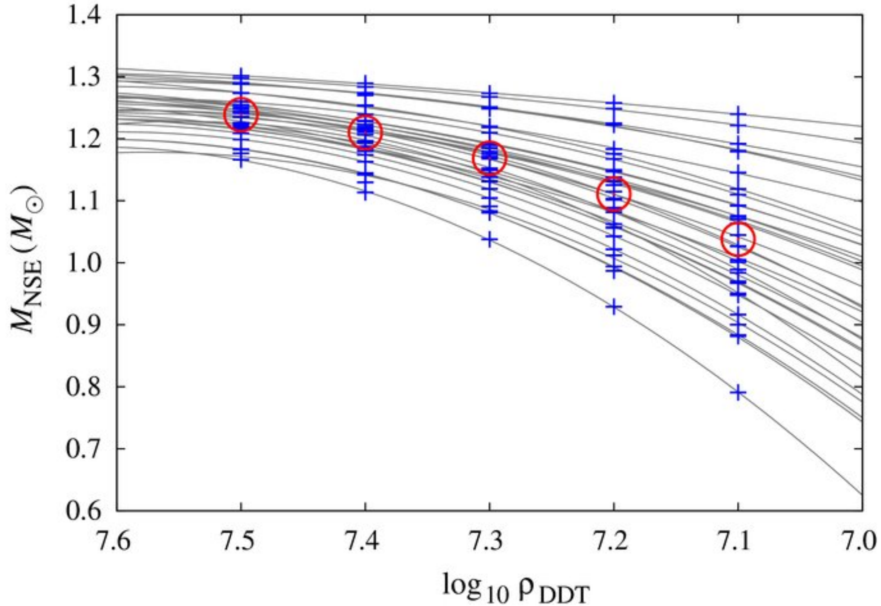
Figure 7. from Evaluating Systematic Dependencies of Type Ia Supernovae: The Influence of Deflagration to Detonation Density JACKSON ET AL. 2010 ApJ 720 99 doi:10.1088/0004-637X/720/1/99 https://dx.doi.org/10.1088/0004-637X/720/1/99 © 2010. The American Astronomical Society. All rights reserved.
