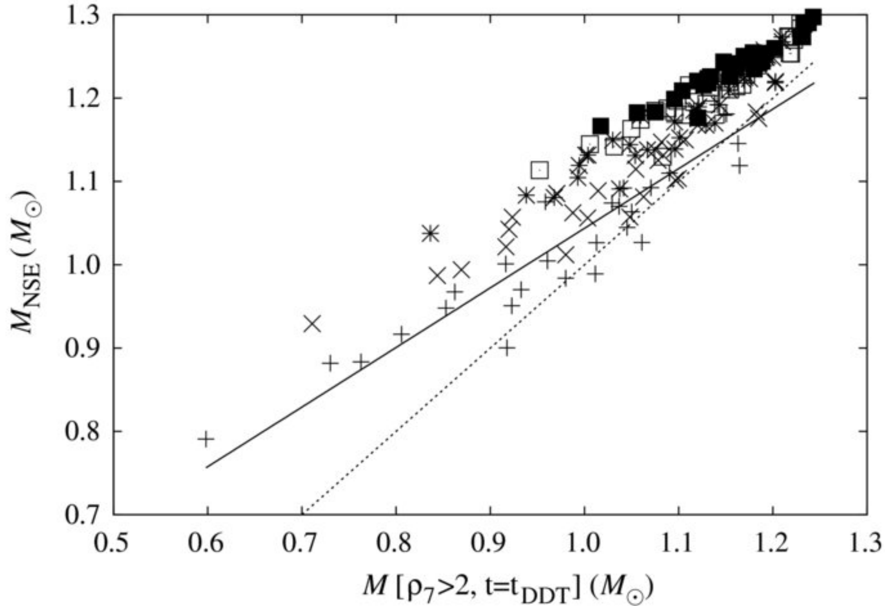
Figure 5. from Evaluating Systematic Dependencies of Type Ia Supernovae: The Influence of Deflagration to Detonation Density JACKSON ET AL. 2010 ApJ 720 99 doi:10.1088/0004-637X/720/1/99 https://dx.doi.org/10.1088/0004-637X/720/1/99 © 2010. The American Astronomical Society. All rights reserved.
