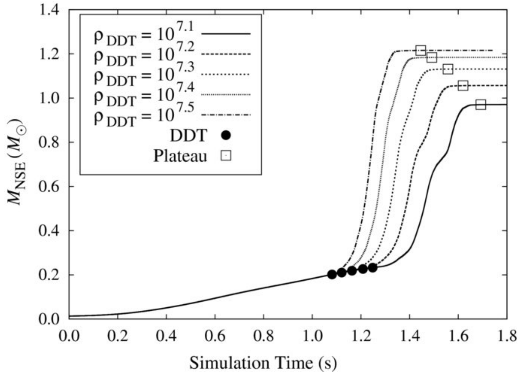
Figure 4. from Evaluating Systematic Dependencies of Type Ia Supernovae: The Influence of Deflagration to Detonation Density JACKSON ET AL. 2010 ApJ 720 99 doi:10.1088/0004-637X/720/1/99 https://dx.doi.org/10.1088/0004-637X/720/1/99 © 2010. The American Astronomical Society. All rights reserved.
