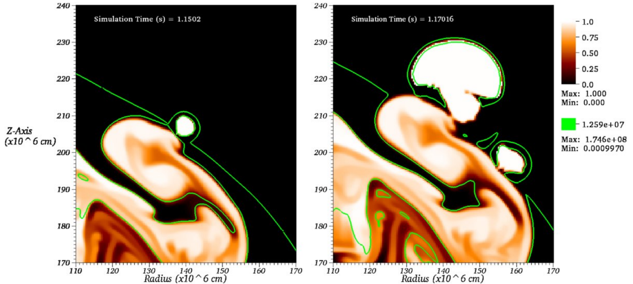
Figure 2. from Evaluating Systematic Dependencies of Type Ia Supernovae: The Influence of Deflagration to Detonation Density JACKSON ET AL. 2010 ApJ 720 99 doi:10.1088/0004-637X/720/1/99 https://dx.doi.org/10.1088/0004-637X/720/1/99 © 2010. The American Astronomical Society. All rights reserved.
