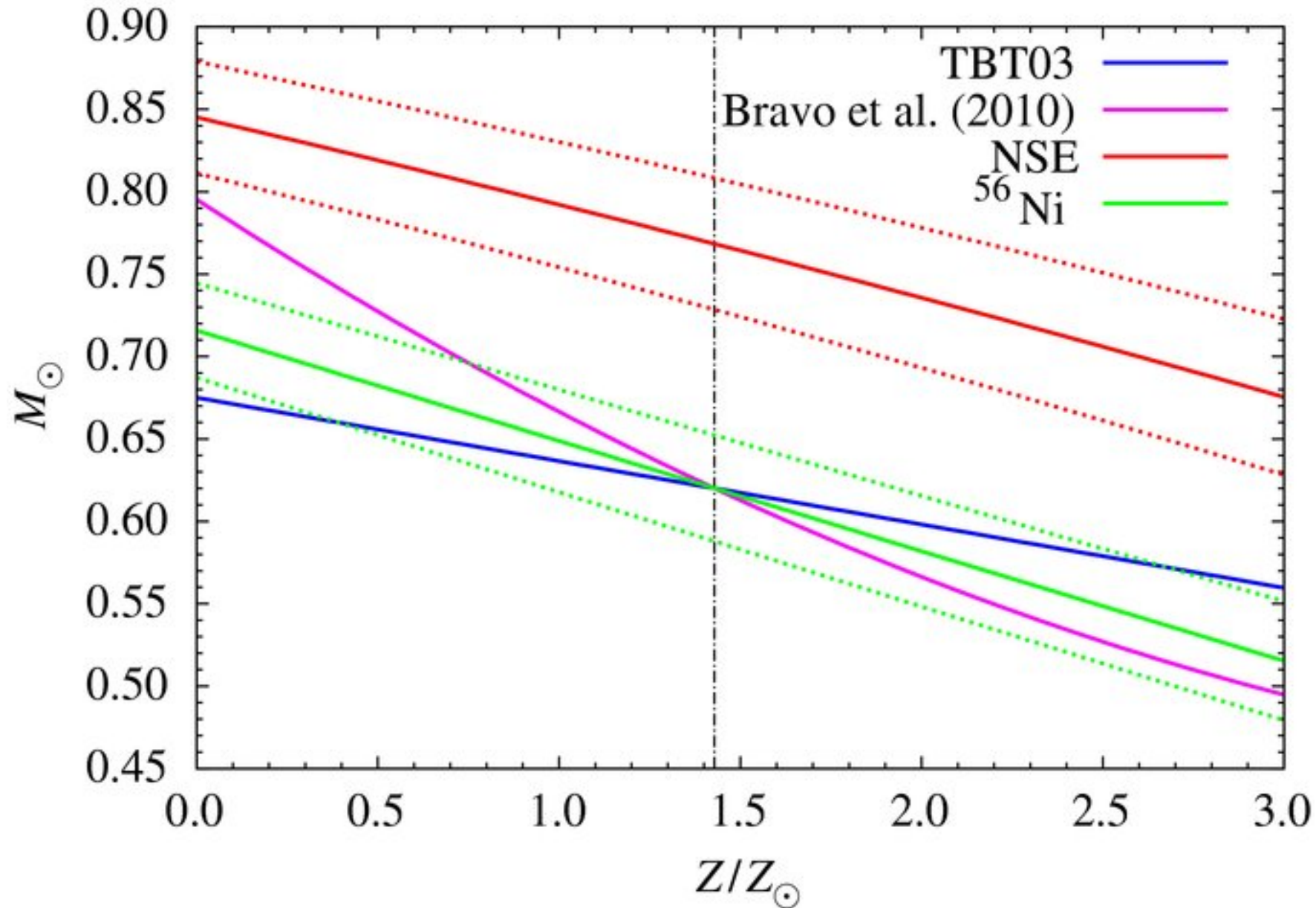
Figure 13. from Evaluating Systematic Dependencies of Type Ia Supernovae: The Influence of Deflagration to Detonation Density JACKSON ET AL. 2010 ApJ 720 99 doi:10.1088/0004-637X/720/1/99 https://dx.doi.org/10.1088/0004-637X/720/1/99 © 2010. The American Astronomical Society. All rights reserved.
