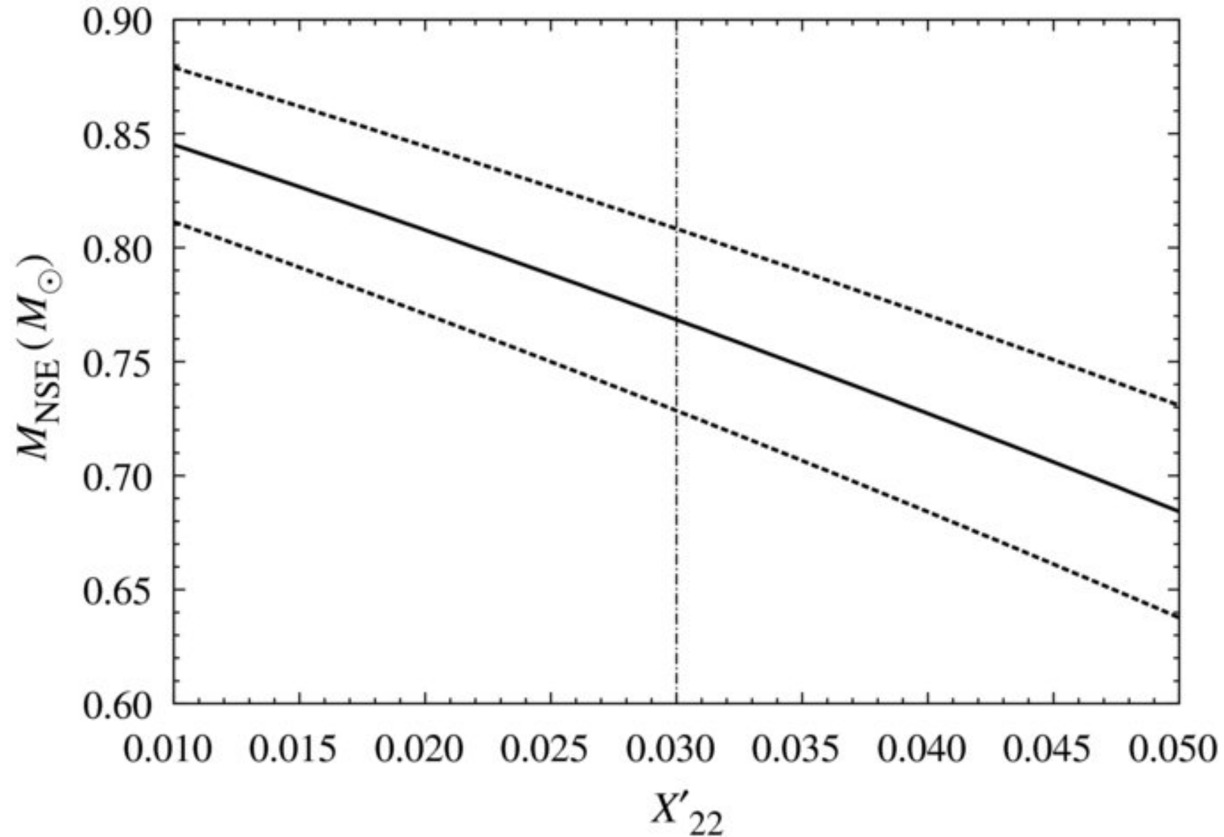
Figure 11. from Evaluating Systematic Dependencies of Type Ia Supernovae: The Influence of Deflagration to Detonation Density JACKSON ET AL. 2010 ApJ 720 99 doi:10.1088/0004-637X/720/1/99 https://dx.doi.org/10.1088/0004-637X/720/1/99 © 2010. The American Astronomical Society. All rights reserved.
