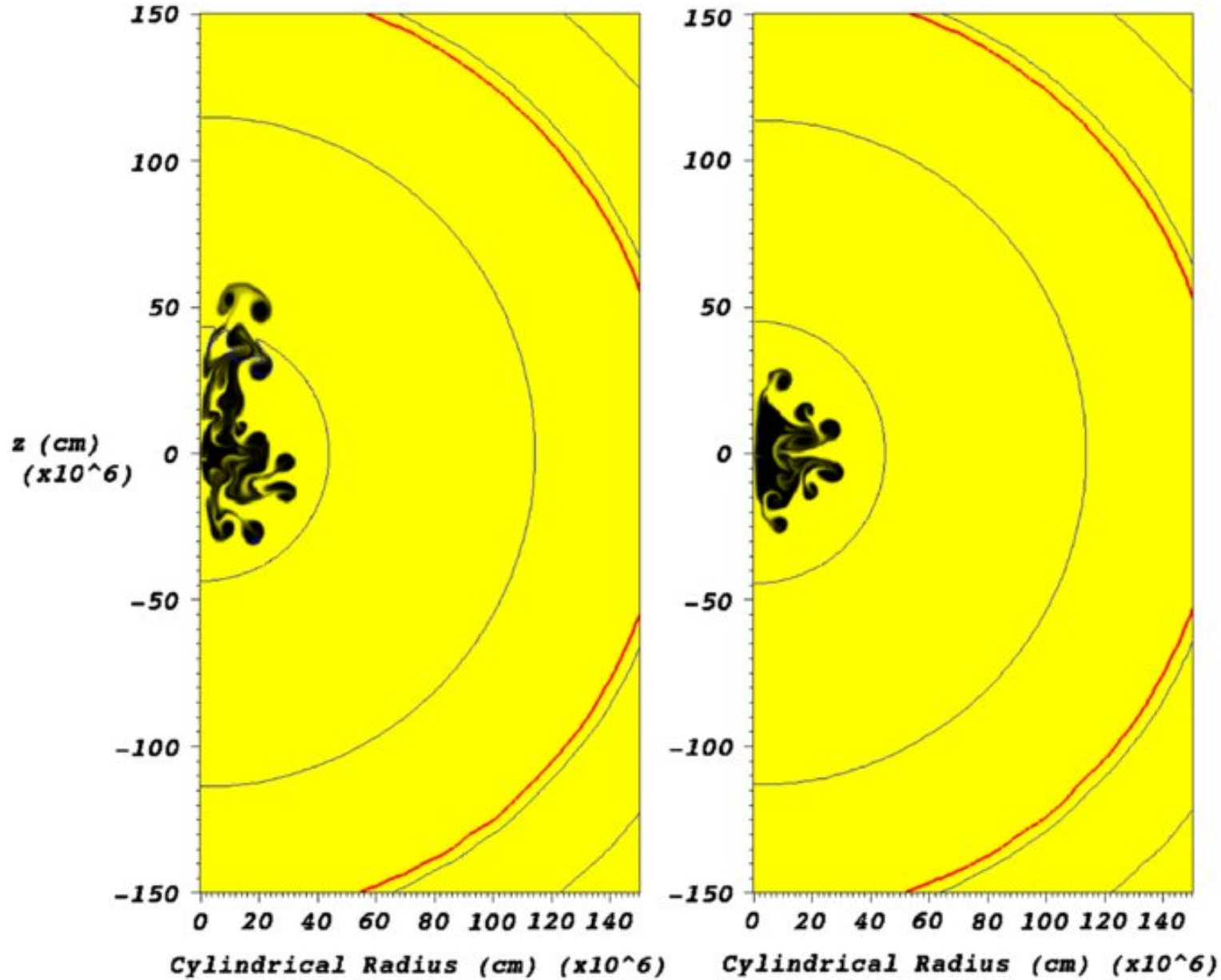
Figure 10. from Evaluating Systematic Dependencies of Type Ia Supernovae: The Influence of Deflagration to Detonation Density JACKSON ET AL. 2010 ApJ 720 99 doi:10.1088/0004-637X/720/1/99 https://dx.doi.org/10.1088/0004-637X/720/1/99 © 2010. The American Astronomical Society. All rights reserved.
