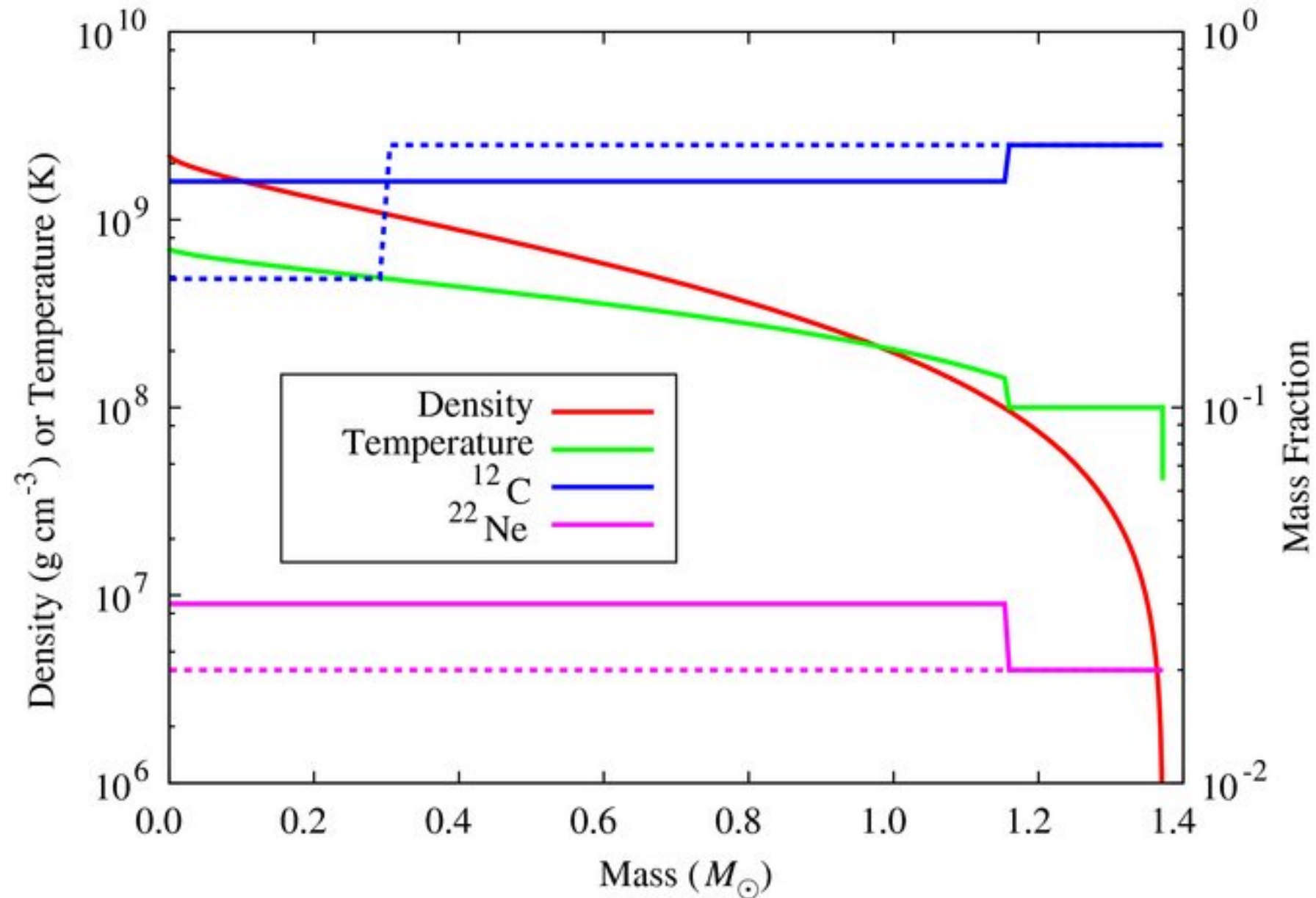
Figure 1. from Evaluating Systematic Dependencies of Type Ia Supernovae: The Influence of Deflagration to Detonation Density JACKSON ET AL. 2010 ApJ 720 99 doi:10.1088/0004-637X/720/1/99 https://dx.doi.org/10.1088/0004-637X/720/1/99 © 2010. The American Astronomical Society. All rights reserved.
