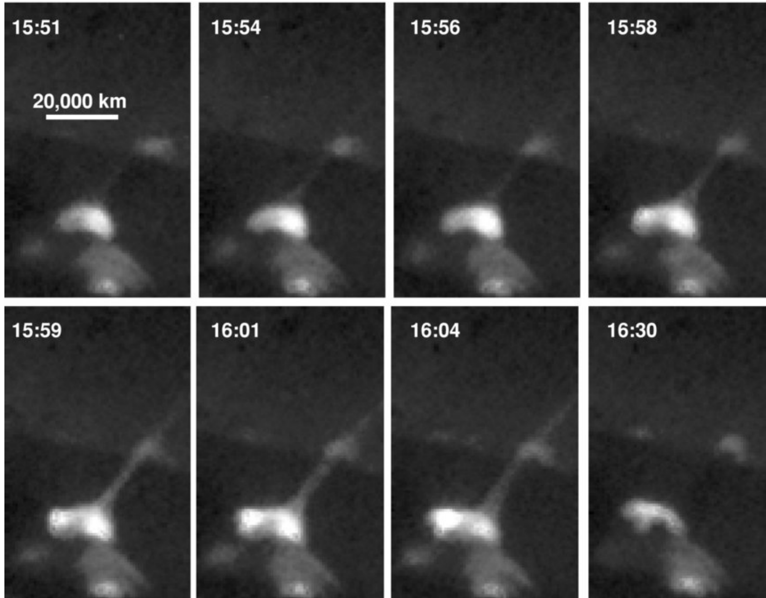
Figure 4. from Dichotomy of Solar Coronal Jets: Standard Jets and Blowout Jets MOORE ET AL. 2010 ApJ 720 757 doi:10.1088/0004-637X/720/1/757 https://dx.doi.org/10.1088/0004-637X/720/1/757 © 2010. The American Astronomical Society. All rights reserved.
