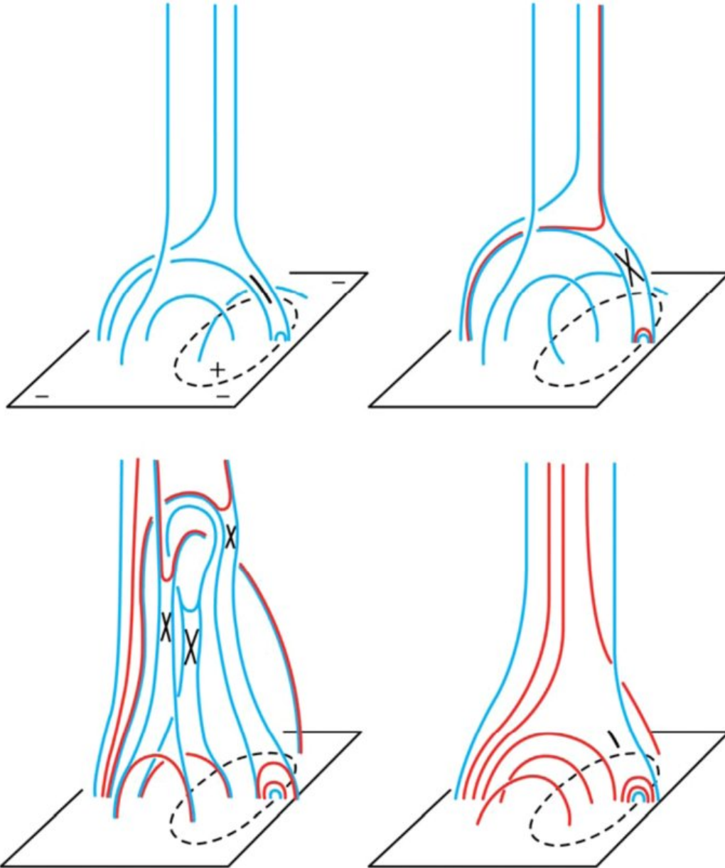
Figure 10. from Dichotomy of Solar Coronal Jets: Standard Jets and Blowout Jets MOORE ET AL. 2010 ApJ 720 757 doi:10.1088/0004-637X/720/1/757 https://dx.doi.org/10.1088/0004-637X/720/1/757 © 2010. The American Astronomical Society. All rights reserved.
