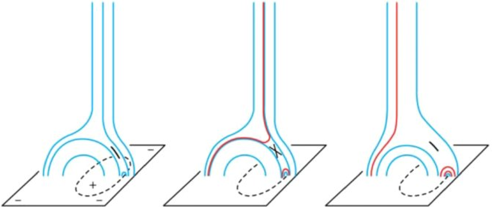
Figure 1. from Dichotomy of Solar Coronal Jets: Standard Jets and Blowout Jets MOORE ET AL. 2010 ApJ 720 757 doi:10.1088/0004-637X/720/1/757 https://dx.doi.org/10.1088/0004-637X/720/1/757 © 2010. The American Astronomical Society. All rights reserved.
