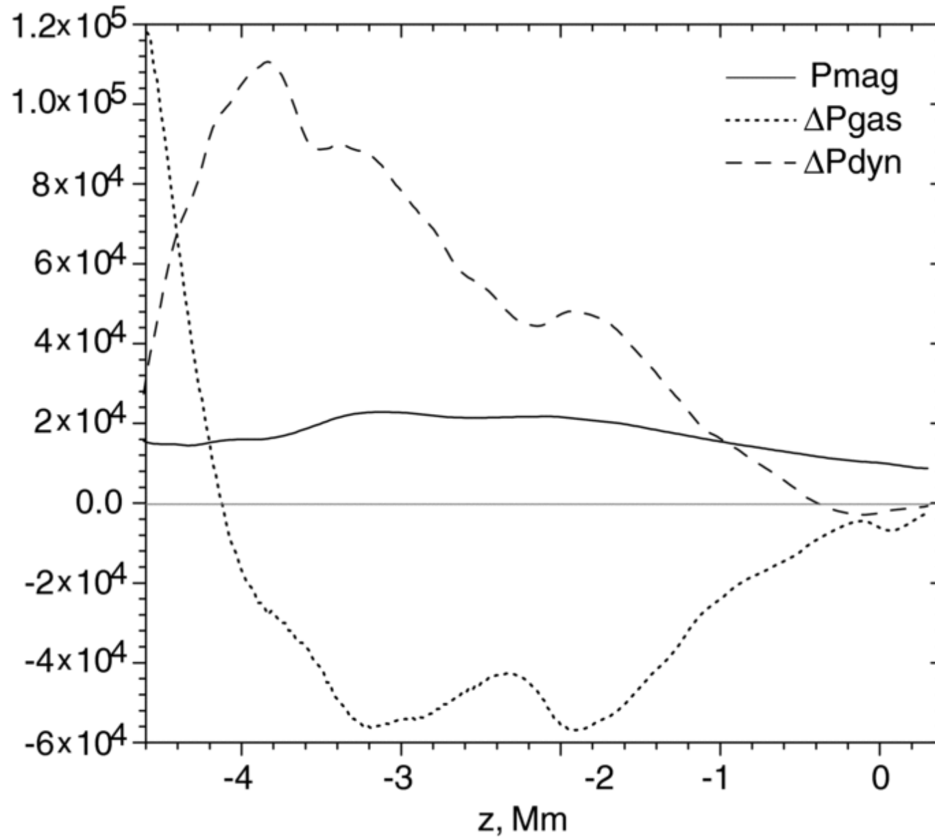
Figure 5. from Mechanism of Spontaneous Formation of Stable Magnetic Structures on the Sun KITIASHVILI ET AL. 2010 ApJ 719 307 doi:10.1088/0004-637X/719/1/307 https://dx.doi.org/10.1088/0004-637X/719/1/307 © 2010. The American Astronomical Society. All rights reserved.
