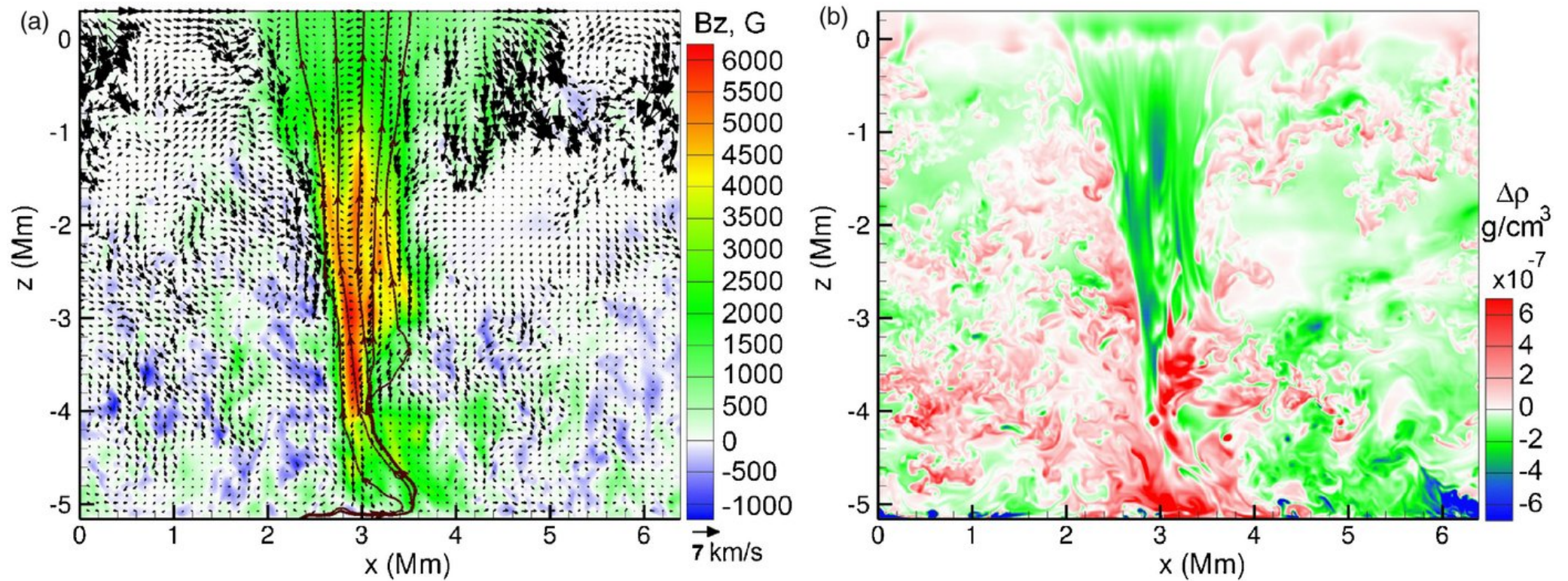
Figure 4. from Mechanism of Spontaneous Formation of Stable Magnetic Structures on the Sun KITIAHVILI ET AL. 2010 ApJ 719 307 doi:10.1088/0004-637X/719/1/307 https://dx.doi.org/10.1088/0004-637X/719/1/307 © 2010. The American Astronomical Society. All rights reserved.
