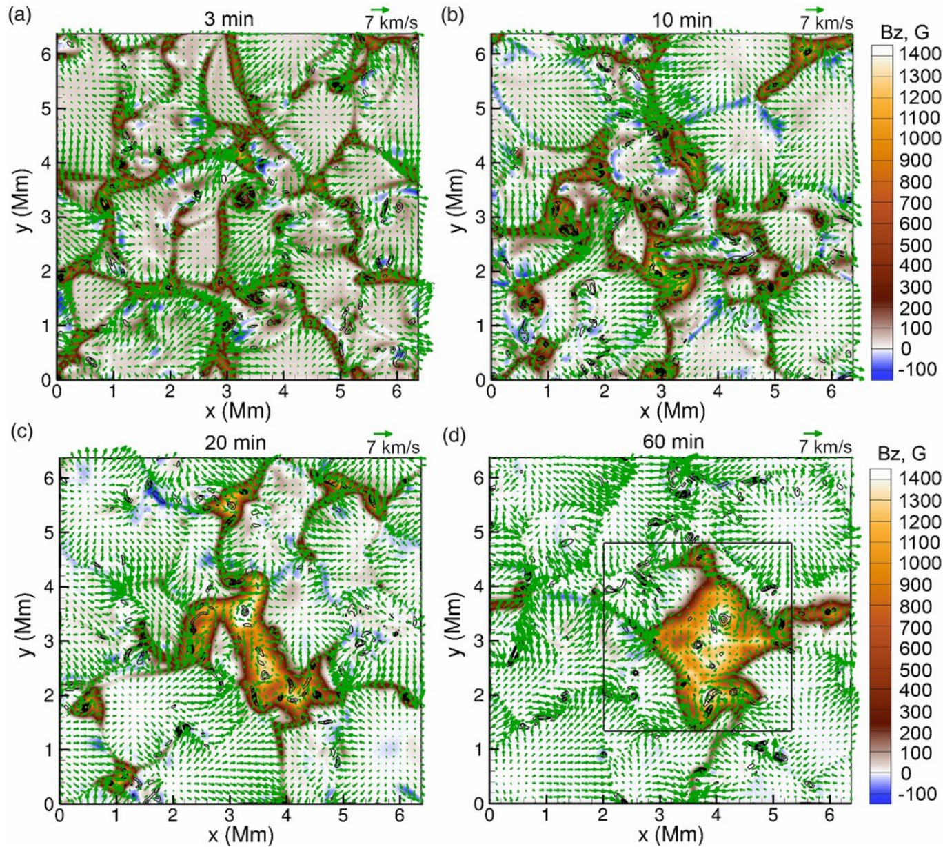
Figure 2. from Mechanism of Spontaneous Formation of Stable Magnetic Structures on the Sun KITIASHVILI ET AL. 2010 ApJ 719 307 doi:10.1088/0004-637X/719/1/307 https://dx.doi.org/10.1088/0004-637X/719/1/307 © 2010. The American Astronomical Society. All rights reserved.
