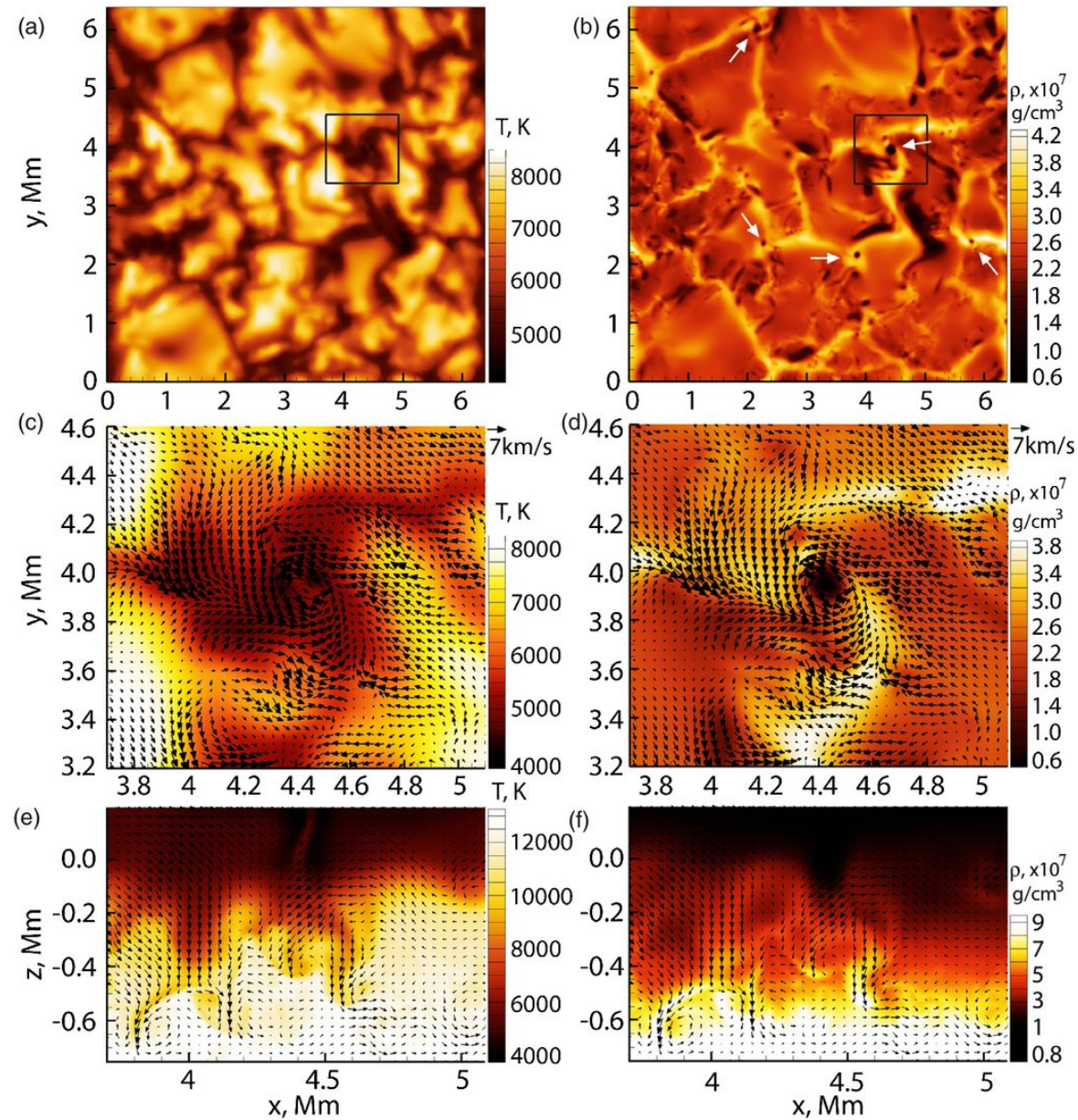
Figure 1. from Mechanism of Spontaneous Formation of Stable Magnetic Structures on the Sun KITIAHVILI ET AL. 2010 ApJ 719 307 doi:10.1088/0004-637X/719/1/307 https://dx.doi.org/10.1088/0004-637X/719/1/307 © 2010. The American Astronomical Society. All rights reserved.
