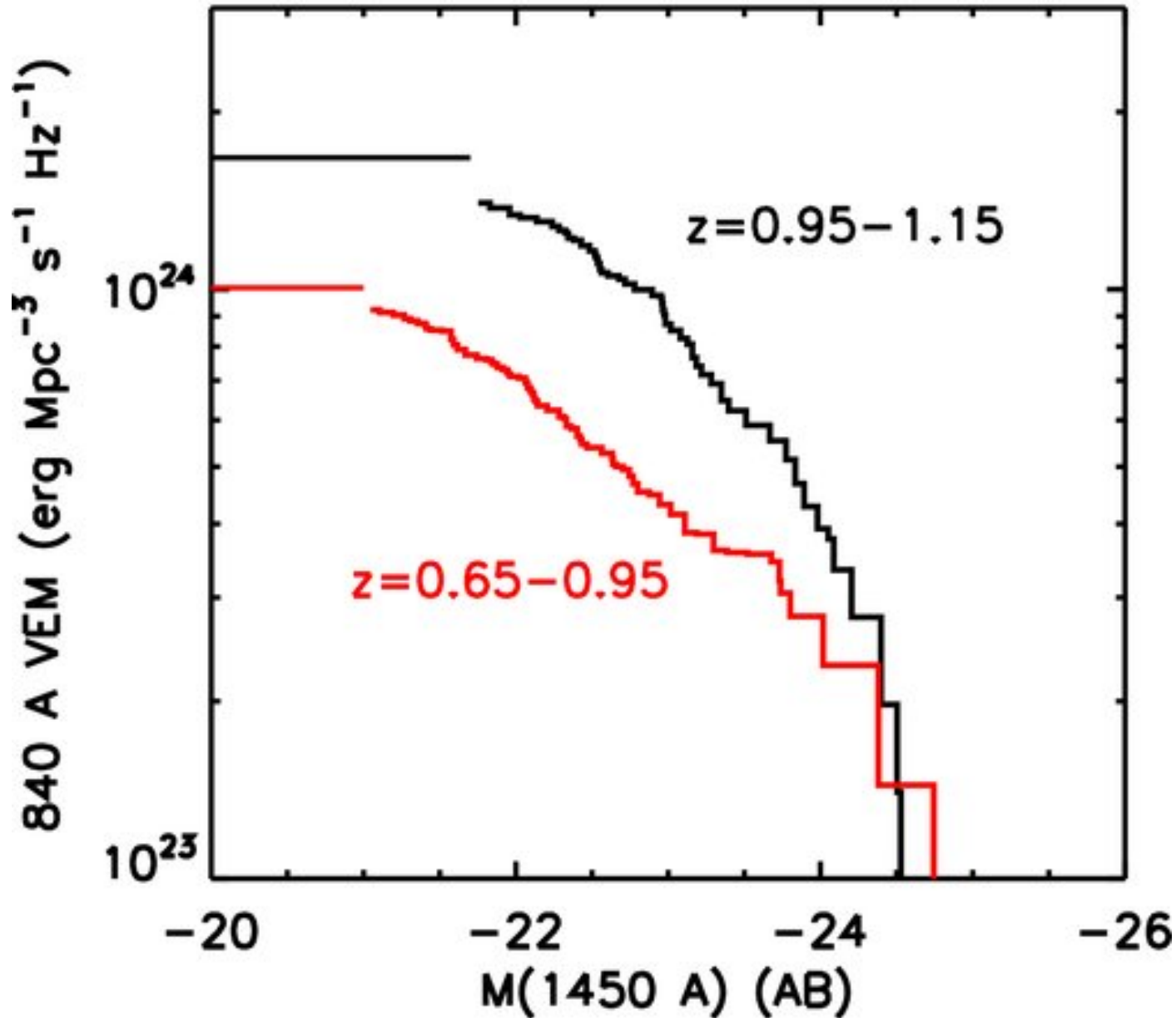
Figure 4. from Active Galactic Nuclei Selected from GALEX Spectroscopy: The Ionizing Source Spectrum at z \sim 1 BARGER & COWIE 2010 ApJ 718 1235 doi:10.1088/0004-637X/718/2/1235 https://dx.doi.org/10.1088/0004-637X/718/2/1235 © 2010. The American Astronomical Society. All rights reserved.
