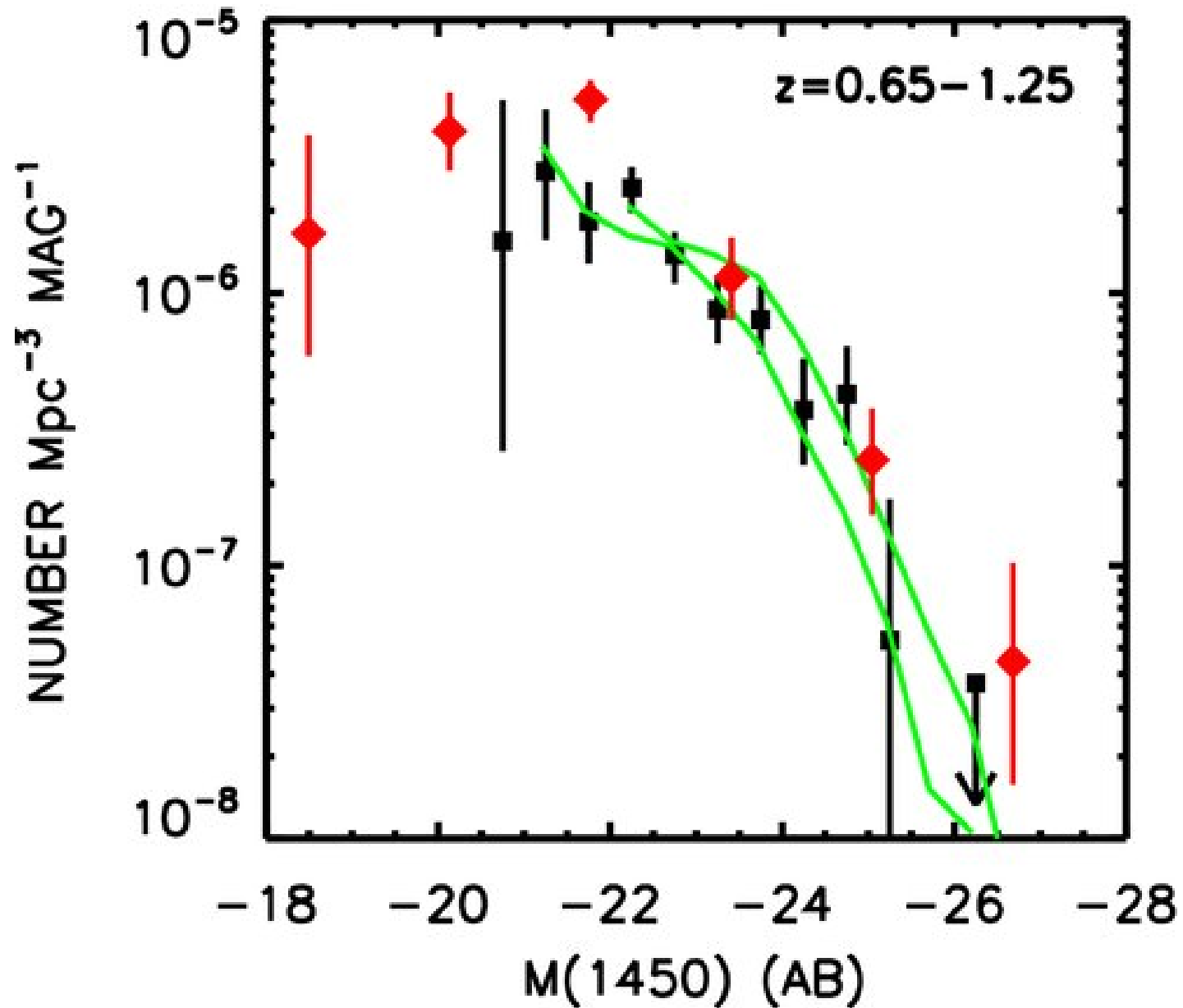
Figure 2. from Active Galactic Nuclei Selected from GALEX Spectroscopy: The Ionizing Source Spectrum at z \sim 1 BARGER & COWIE 2010 ApJ 718 1235 doi:10.1088/0004-637X/718/2/1235 https://dx.doi.org/10.1088/0004-637X/718/2/1235 © 2010. The American Astronomical Society. All rights reserved.
