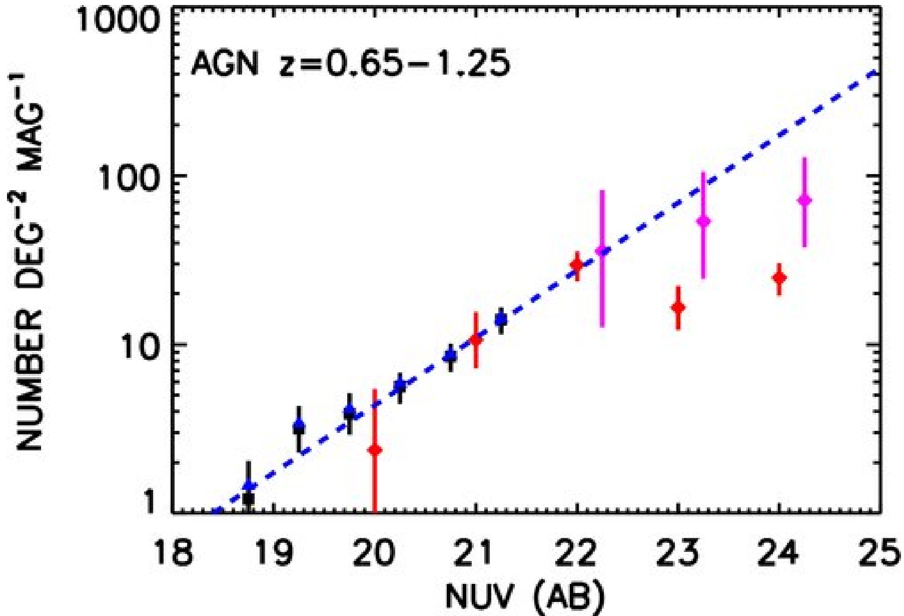
Figure 1. from Active Galactic Nuclei Selected from GALEX Spectroscopy: The Ionizing Source Spectrum at z \sim 1 BARGER & COWIE 2010 ApJ 718 1235 doi:10.1088/0004-637X/718/2/1235 https://dx.doi.org/10.1088/0004-637X/718/2/1235 © 2010. The American Astronomical Society. All rights reserved.
