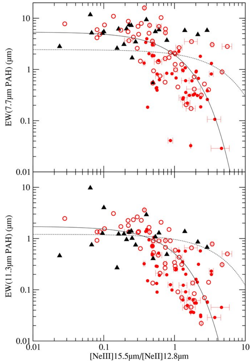
Figure 9. from Polycyclic Aromatic Hydrocarbon and Emission Line Ratios in Active Galactic Nuclei and Starburst Galaxies SALES, PASTORIZA, & RIFFEL 2010 ApJ 725 605 doi:10.1088/0004-637X/725/1/605 https://dx.doi.org/10.1088/0004-637X/725/1/605
