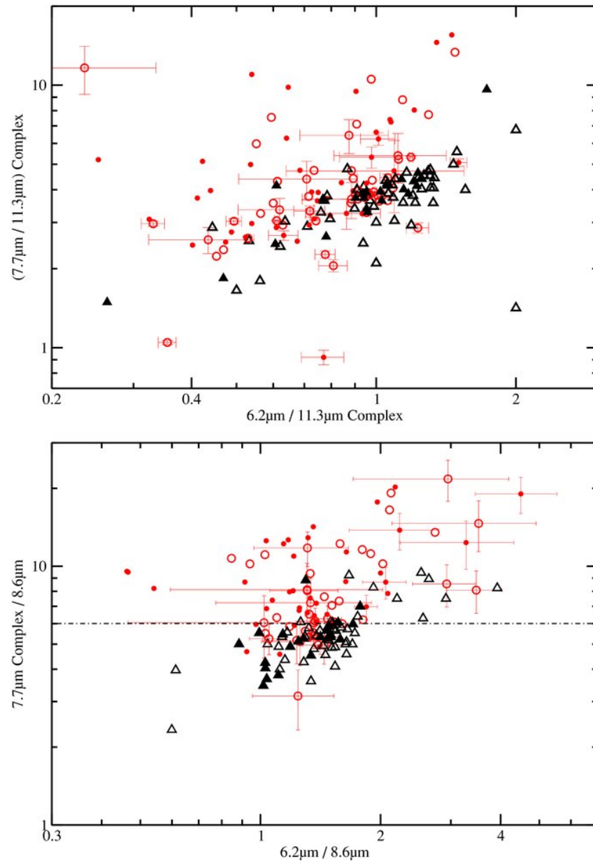
Figure 6. from Polycyclic Aromatic Hydrocarbon and Emission Line Ratios in Active Galactic Nuclei and Starburst Galaxies SALES, PASTORIZA, & RIFFEL 2010 ApJ 725 605 doi:10.1088/0004-637X/725/1/605 https://dx.doi.org/10.1088/0004-637X/725/1/605
