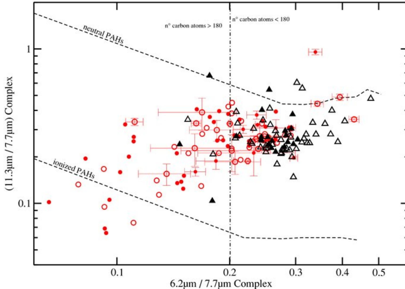
Figure 5. from Polycyclic Aromatic Hydrocarbon and Emission Line Ratios in Active Galactic Nuclei and Starburst Galaxies SALES, PASTORIZA, & RIFFEL 2010 ApJ 725 605 doi:10.1088/0004-637X/725/1/605 https://dx.doi.org/10.1088/0004-637X/725/1/605 © 2010. The American Astronomical Society. All rights reserved.
