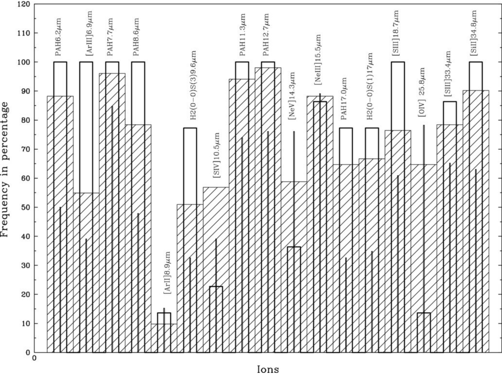
Figure 4. from Polycyclic Aromatic Hydrocarbon and Emission Line Ratios in Active Galactic Nuclei and Starburst Galaxies SALES, PASTORIZA, & RIFFEL 2010 ApJ 725 605 doi:10.1088/0004-637X/725/1/605 https://dx.doi.org/10.1088/0004-637X/725/1/605 © 2010. The American Astronomical Society. All rights reserved.
