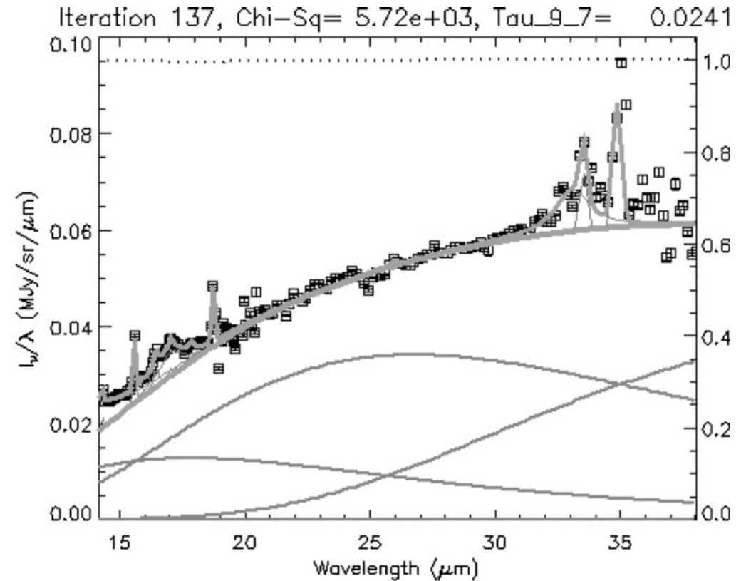
Figure 3. from Polycyclic Aromatic Hydrocarbon and Emission Line Ratios in Active Galactic Nuclei and Starburst Galaxies SALES, PASTORIZA, & RIFFEL 2010 ApJ 725 605 doi:10.1088/0004-637X/725/1/605 https://dx.doi.org/10.1088/0004-637X/725/1/605
