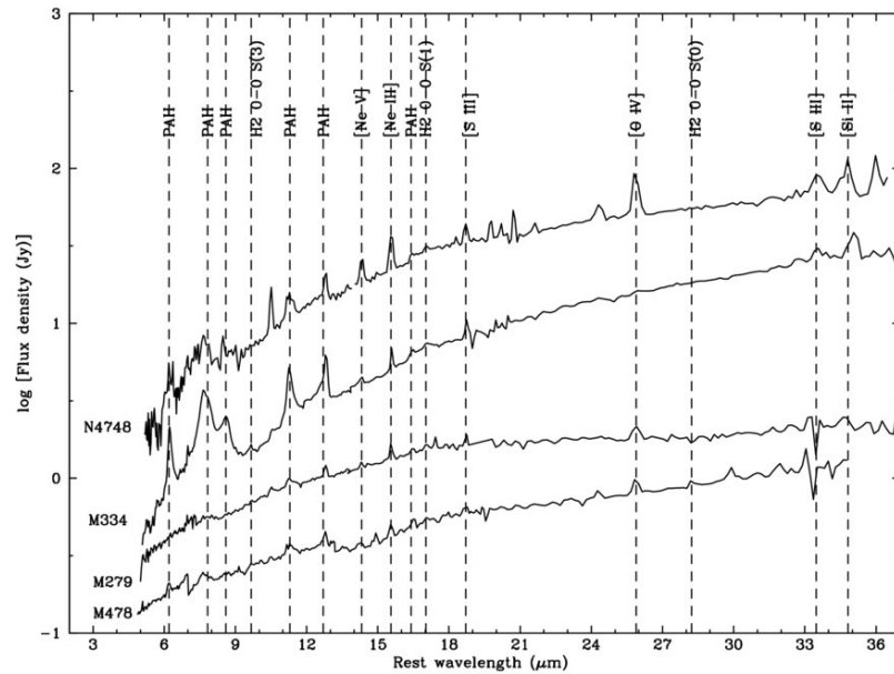
Figure 2. from Polycyclic Aromatic Hydrocarbon and Emission Line Ratios in Active Galactic Nuclei and Starburst Galaxies SALES, PASTORIZA, & RIFFEL 2010 ApJ 725 605 doi:10.1088/0004-637X/725/1/605 https://dx.doi.org/10.1088/0004-637X/725/1/605
