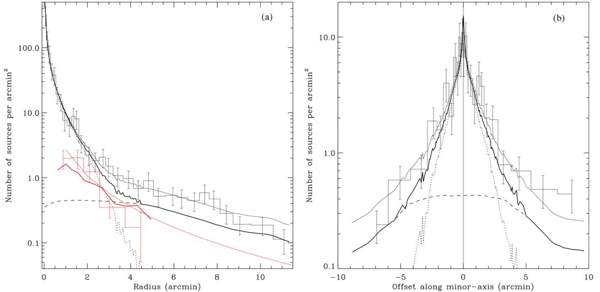
Figure 6. from X-ray Emission from the Sombrero Galaxy: Discrete Sources LI ET AL. 2010 ApJ 721 1368 doi:10.1088/0004-637X/721/2/1368 https://dx.doi.org/10.1088/0004-637X/721/2/1368 © 2010. The American Astronomical Society. All rights reserved.
