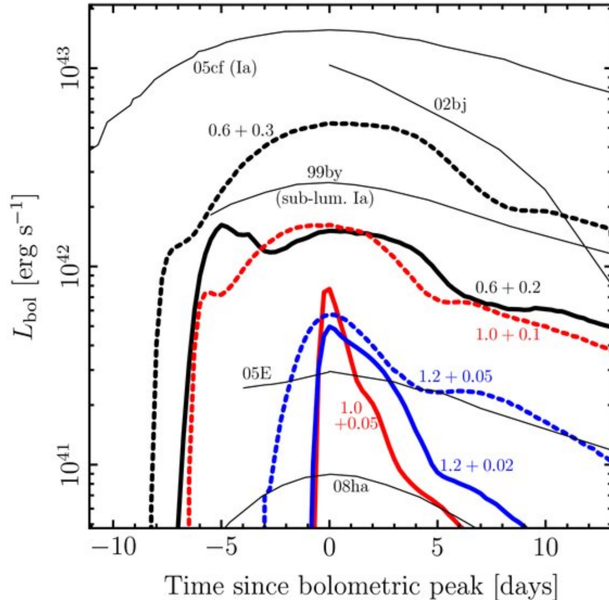
Figure 9. from Thermonuclear .Ia Supernovae from Helium Shell Detonations: Explosion Models and Observables SHEN ET AL. 2010 ApJ 715 767 doi:10.1088/0004-637X/715/2/767 https://dx.doi.org/10.1088/0004-637X/715/2/767 © 2010. The American Astronomical Society. All rights reserved.
