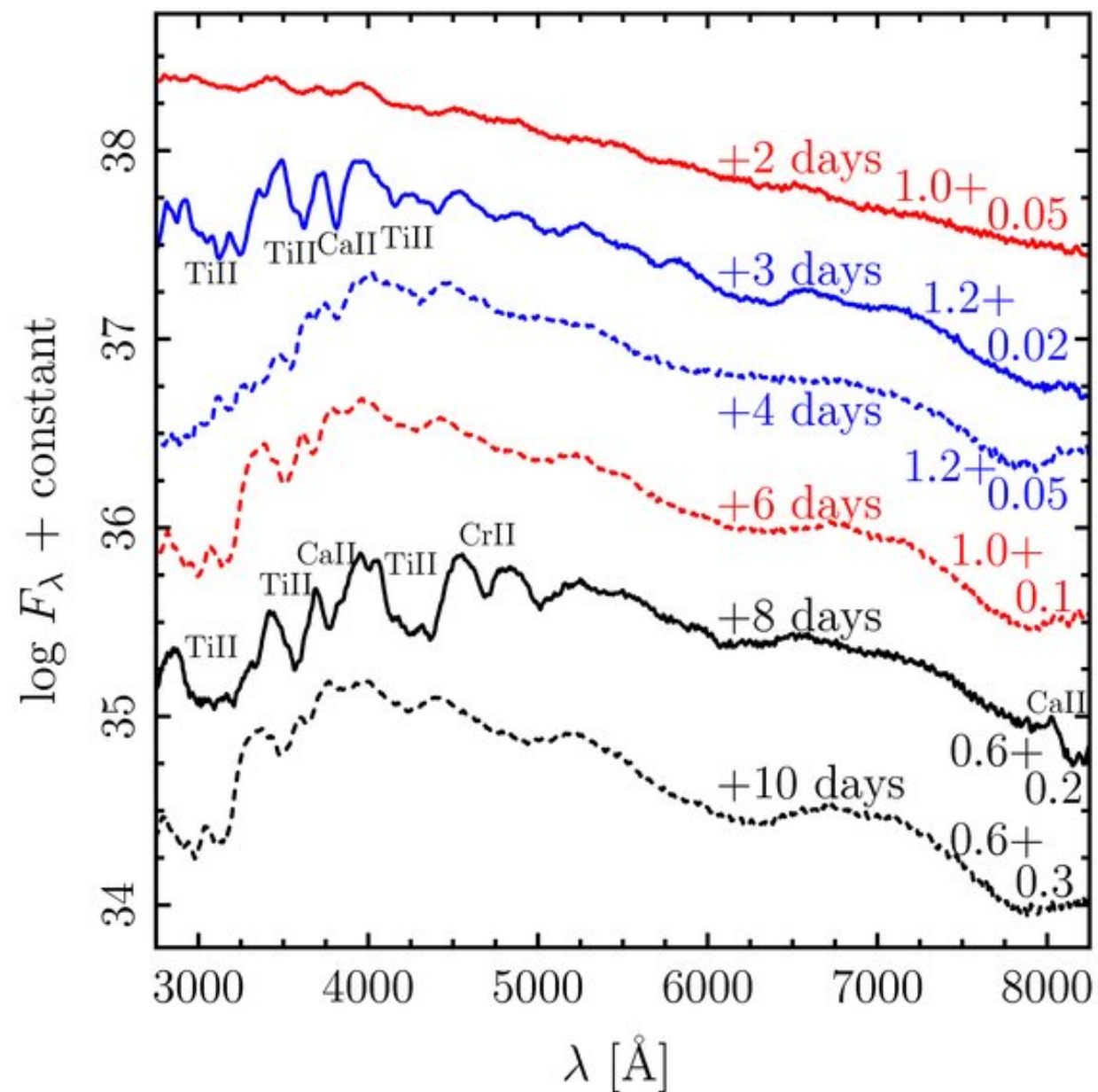
Figure 8. from Thermonuclear .Ia Supernovae from Helium Shell Detonations: Explosion Models and Observables SHEN ET AL. 2010 ApJ 715 767 doi:10.1088/0004-637X/715/2/767 https://dx.doi.org/10.1088/0004-637X/715/2/767 © 2010. The American Astronomical Society. All rights reserved.
