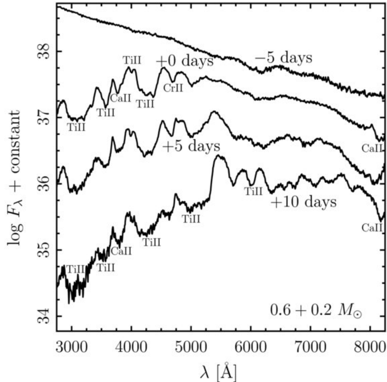
Figure 7. from Thermonuclear .Ia Supernovae from Helium Shell Detonations: Explosion Models and Observables SHEN ET AL. 2010 ApJ 715 767 doi:10.1088/0004-637X/715/2/767 https://dx.doi.org/10.1088/0004-637X/715/2/767 © 2010. The American Astronomical Society. All rights reserved.
